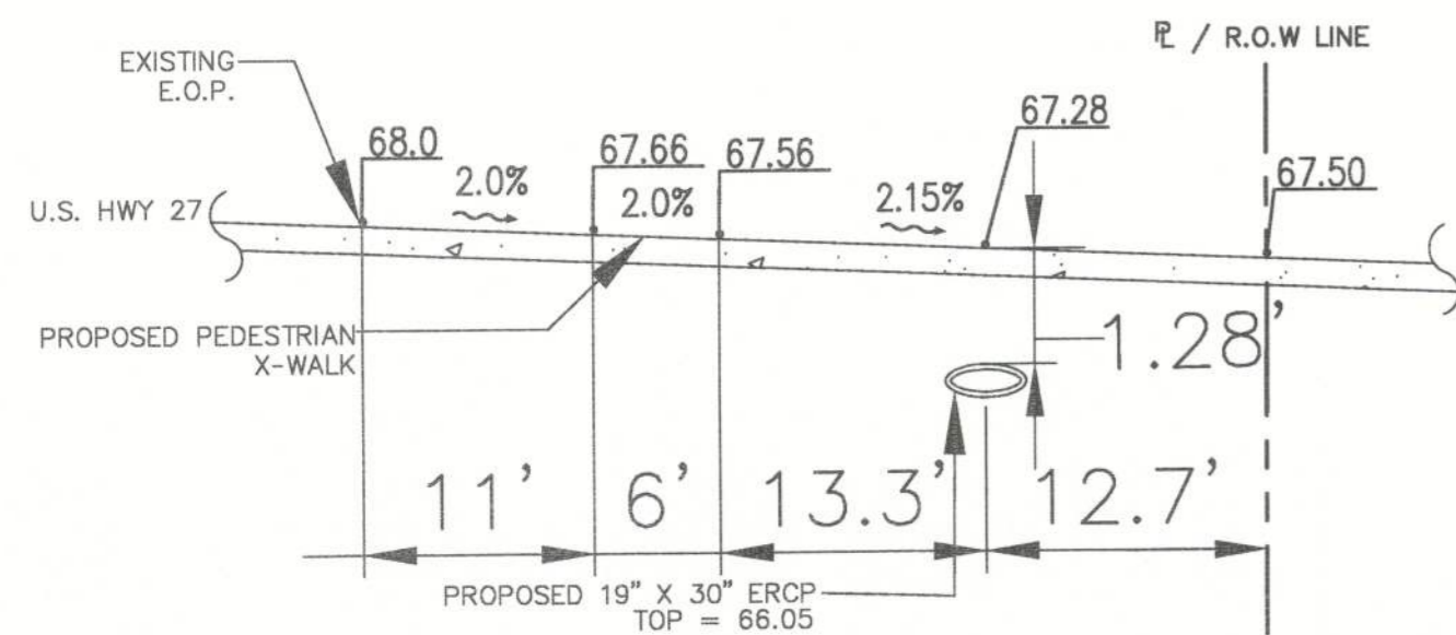
1 DRIVEWAY PROFILE N.T.S.
