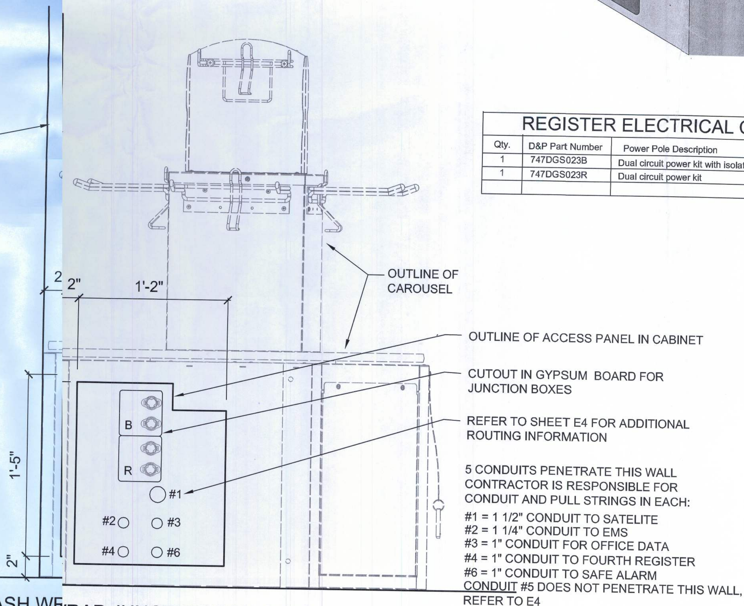
POWER POLE & POWER TERMINAL DETAILS
