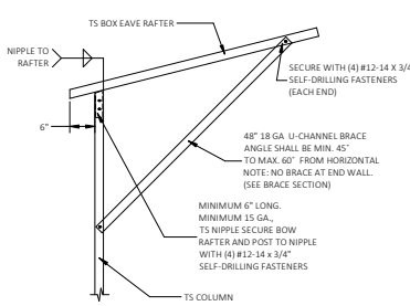
1.1 BOX EAVE RAFTER COLUMN CONNECTION DETAIL FOR HEIGHTS 12'-0" < TO ≤ 13'-0" SCALE: NTS
