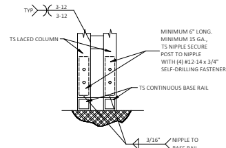
2B SIDEWALL LACED COLUMN/BASE RAIL CONNECTION DETAIL SCALE: NTS
