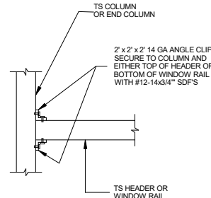
8A NON-STRUCTURAL HEADER OR WINDOW RAIL TO POST CONNECTION DETAIL SCALE: NTS
