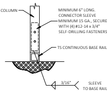
2 SIDEWALL SINGLE COLUMN/BASE RAIL CONNECTION DETAIL SCALE: NTS
