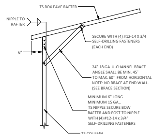
1.2 BOX EAVE RAFTER COLUMN CONNECTION DETAIL FOR HEIGHTS 12'-0" < TO ≤ 13'-0" SCALE: NTS
