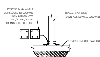
2C ENDWALL COLUMN/BASE RAIL CONNECTION DETAIL SCALE: NTS
