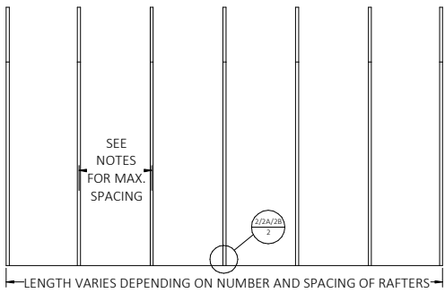
TYPICAL RAFTER/COLUMN SIDE WALL FRAME SECTION
