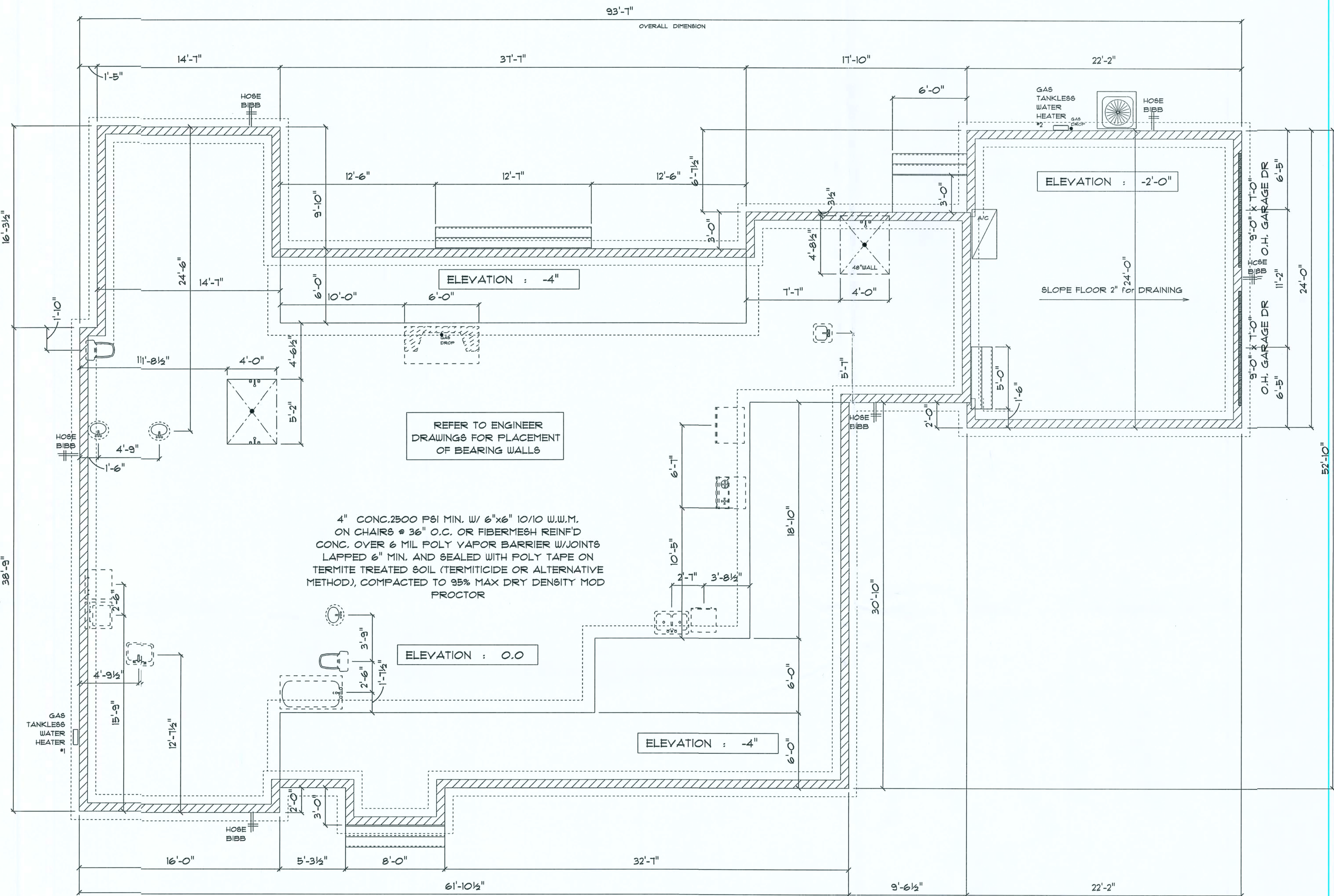
* FLOOR PLAN *
