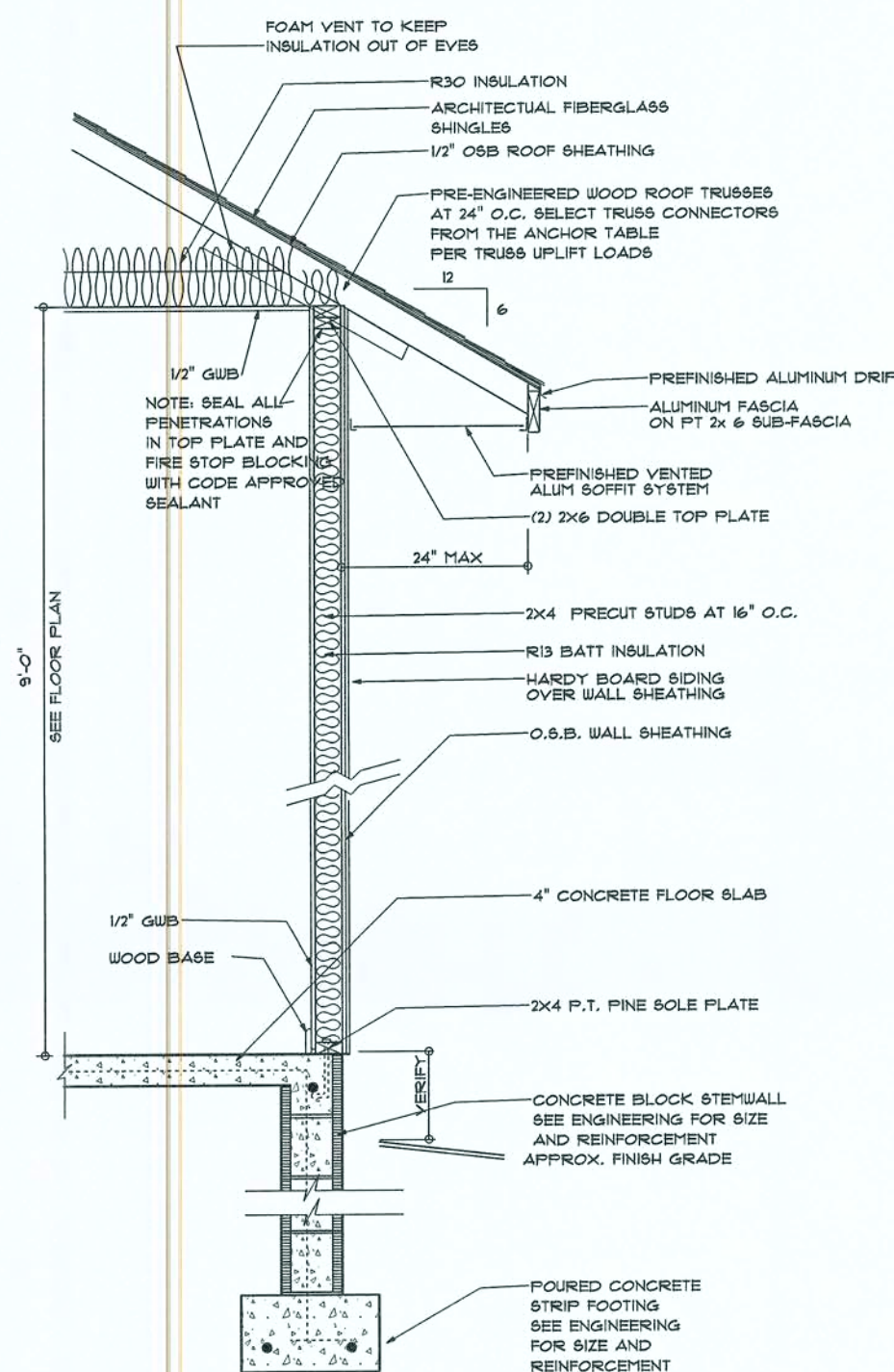
TYPICAL DESIGN WALL SECTION NON - STRUCTURAL DATA
