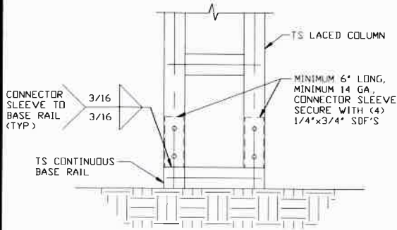
POST/BASE RAIL CONNECTION DETAIL
