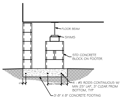
CONCRETE FOOTING DETAIL A-A
