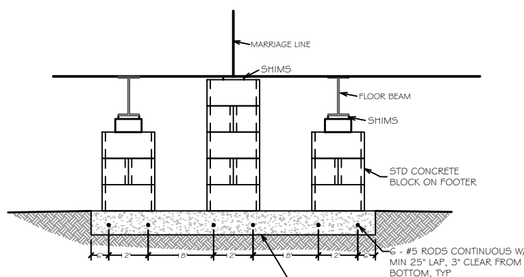
CONCRETE FOOTING DETAIL B-B
