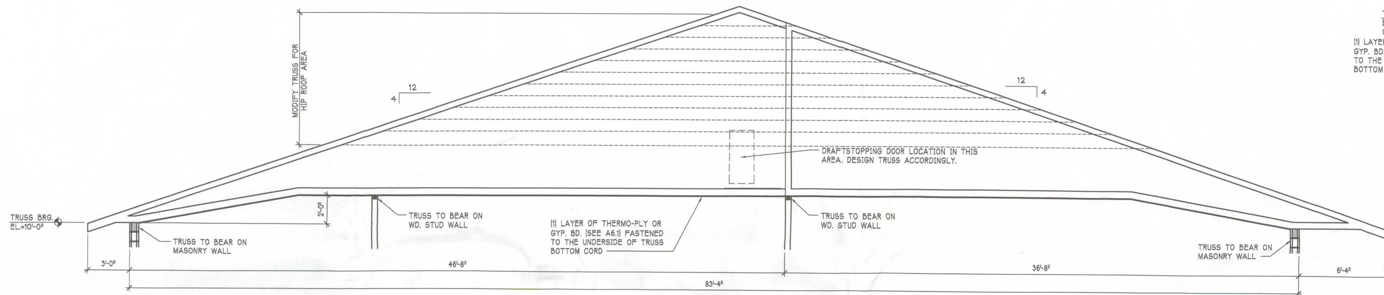
T2 - TRUSS
