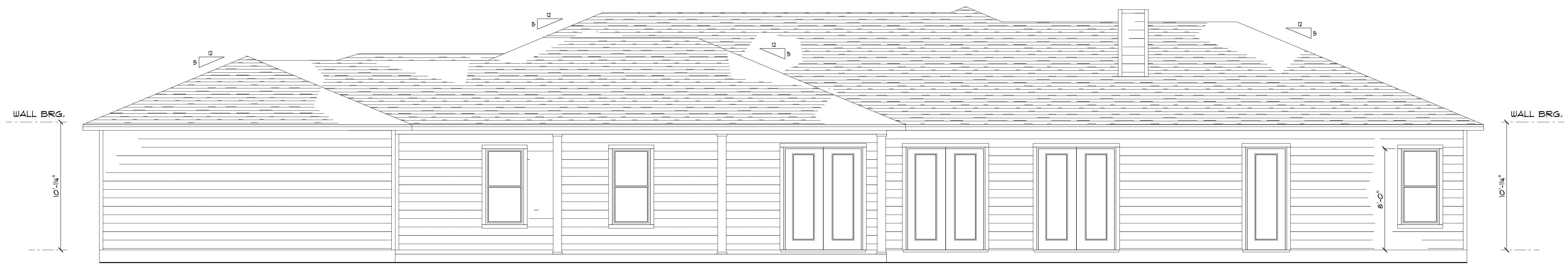
REAR ELEVATION
