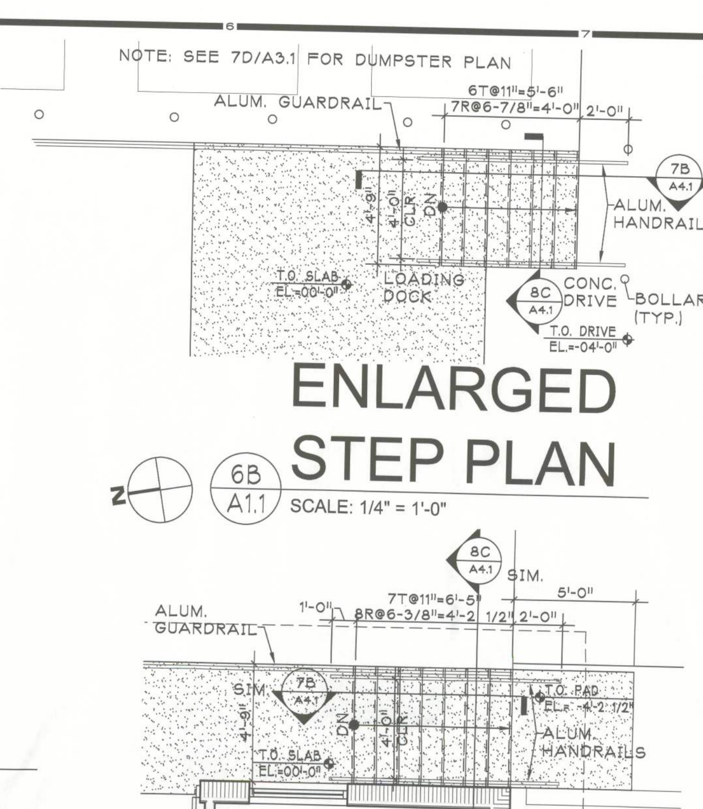
ENLARGED STEP PLAN SCALE: 1/4" = 1'-0"
