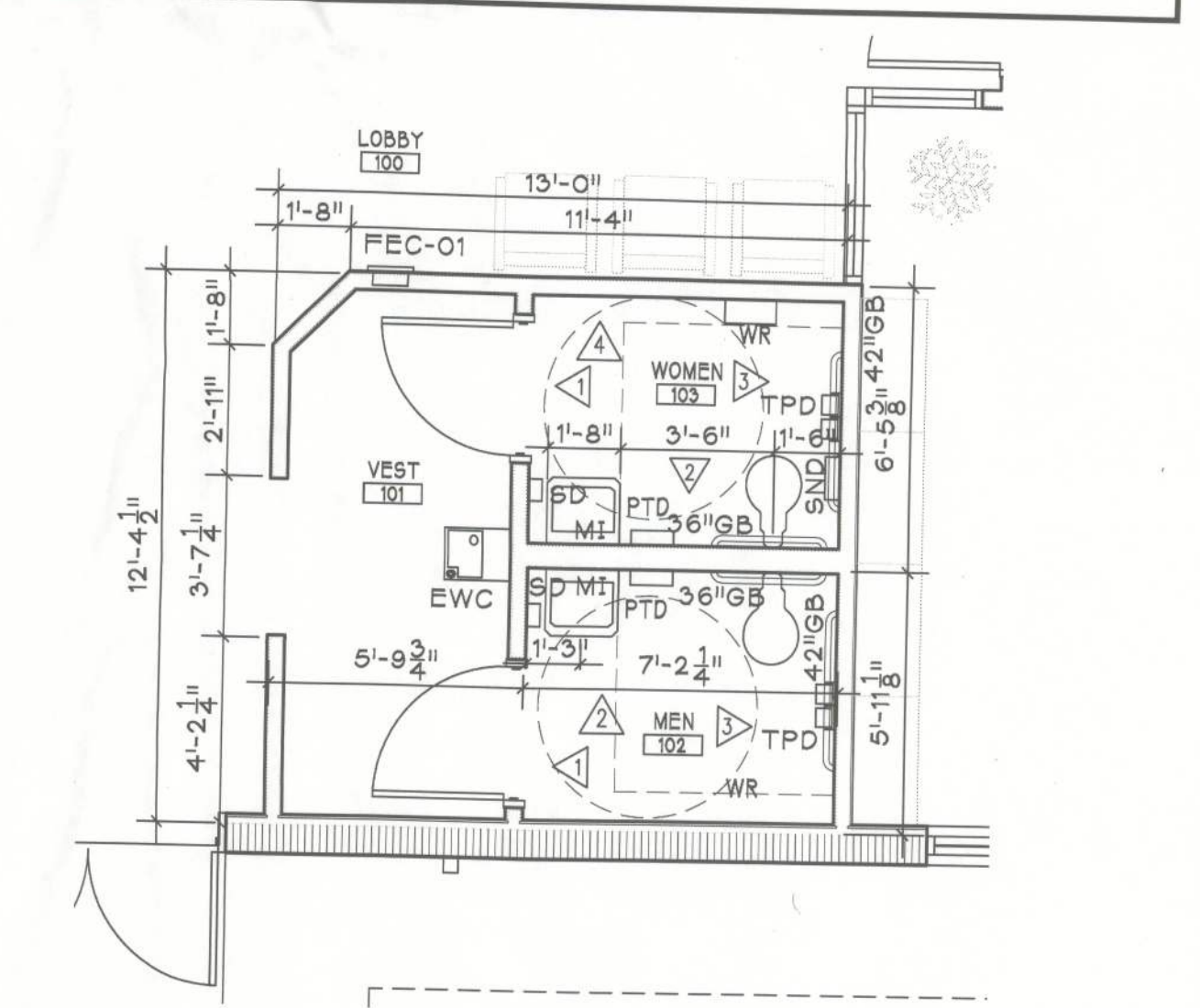
ENLARGED PLAN SCALE: 1/4" = 1'-0"
