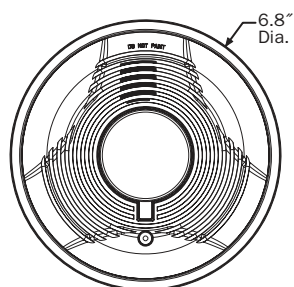
Ceiling-Mount Horn Strobes
