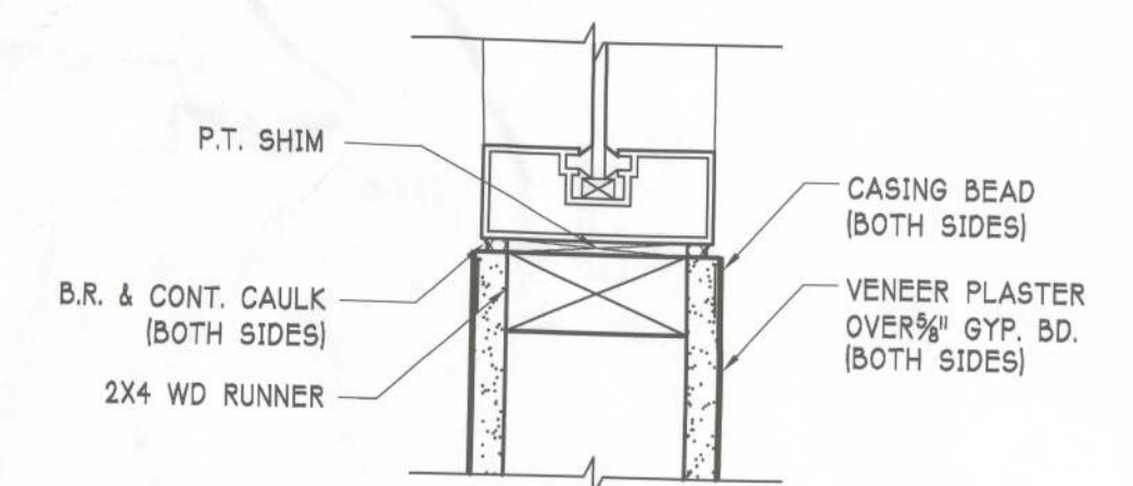
INT. WINDOW SILL
