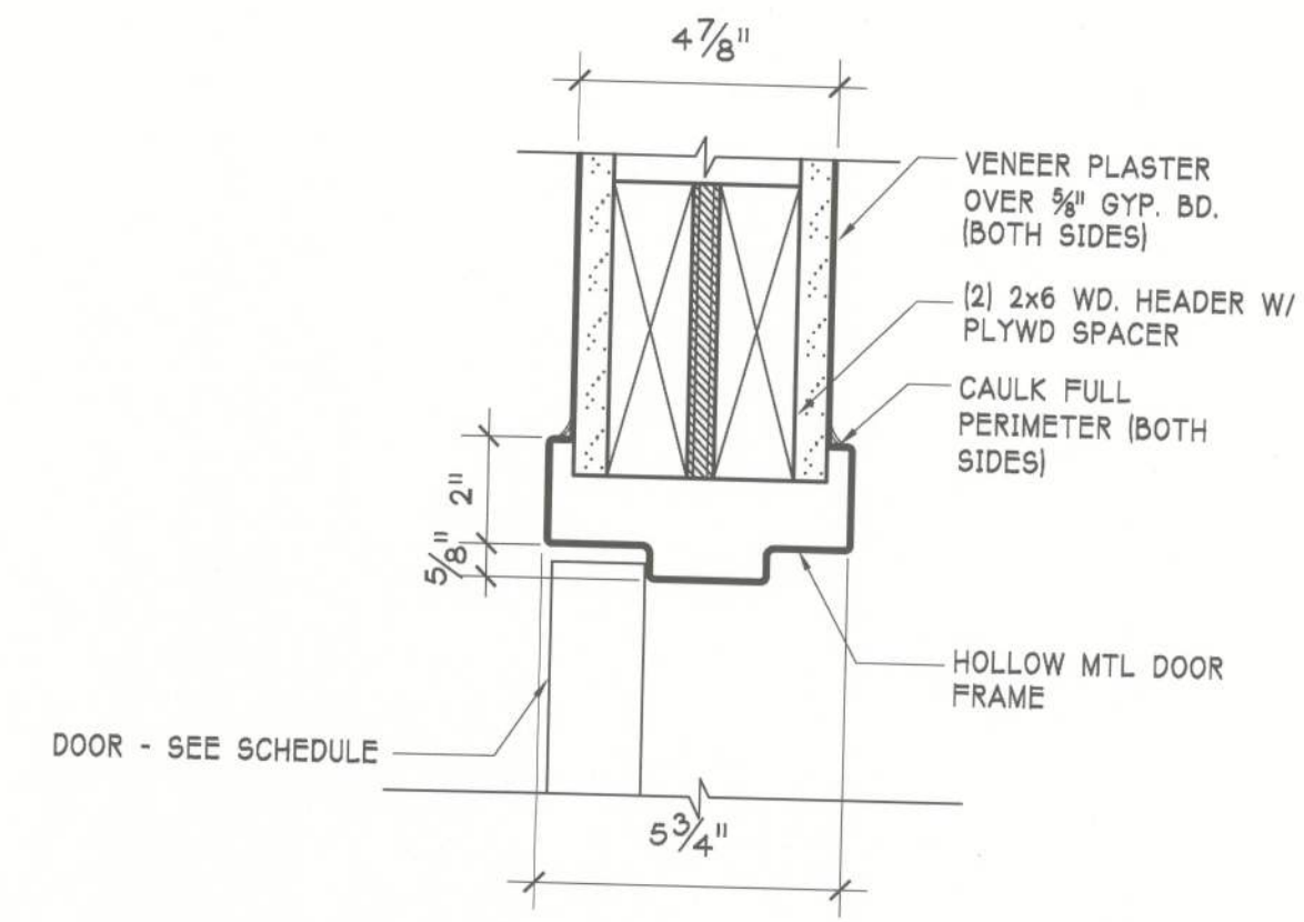
TYPICAL INT. DOOR HEAD HM FRAME/MTL. STUD WALL
