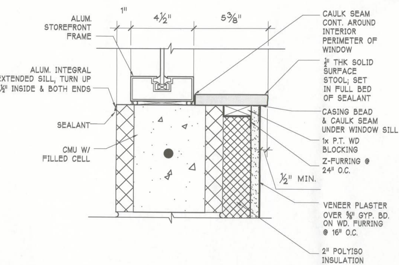
WINDOW SILL / CMU WALL
