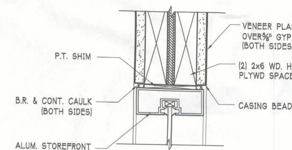
INT. STOREFRONT HEAD
