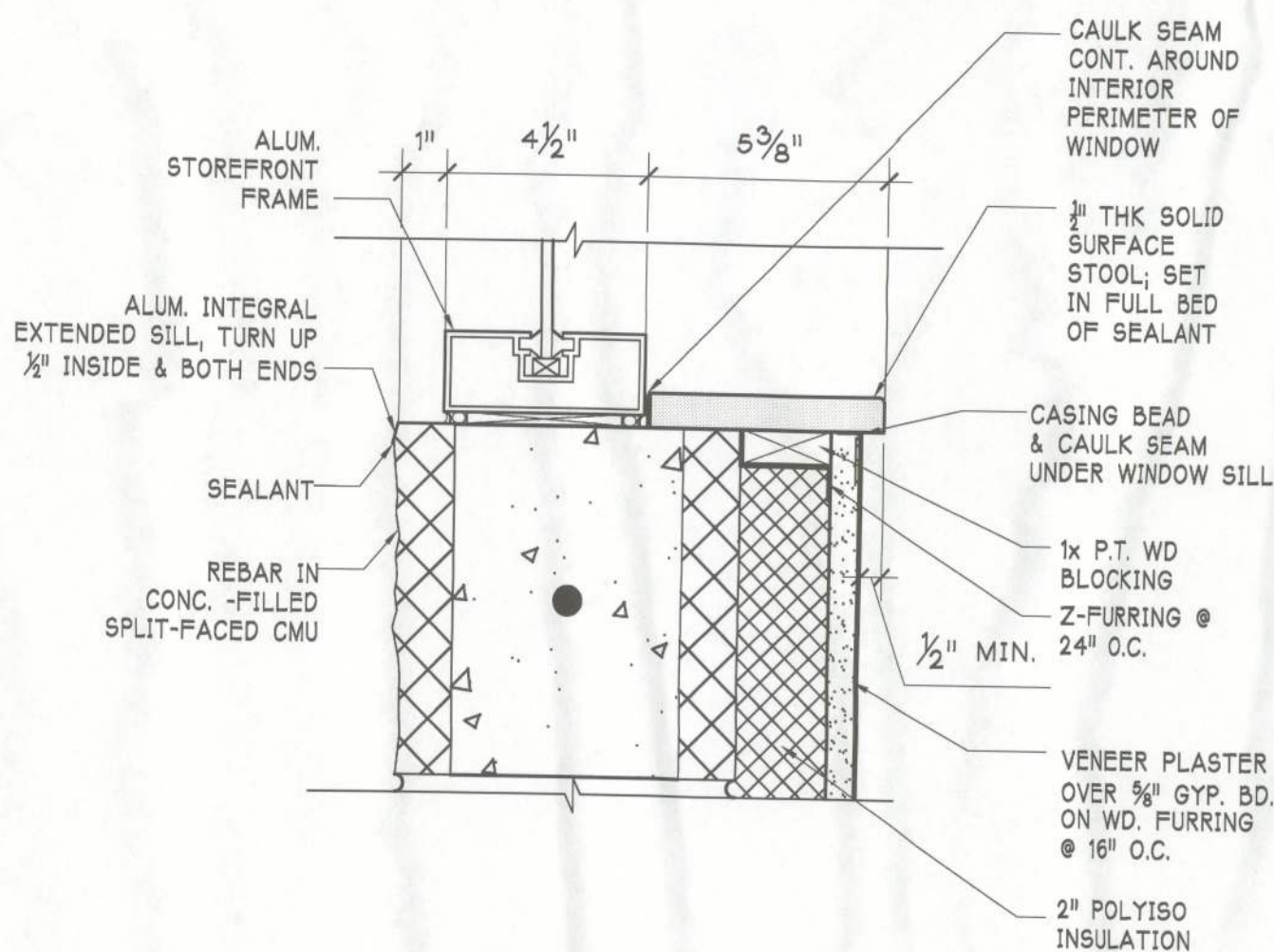
WINDOW SILL / CMU WALL
