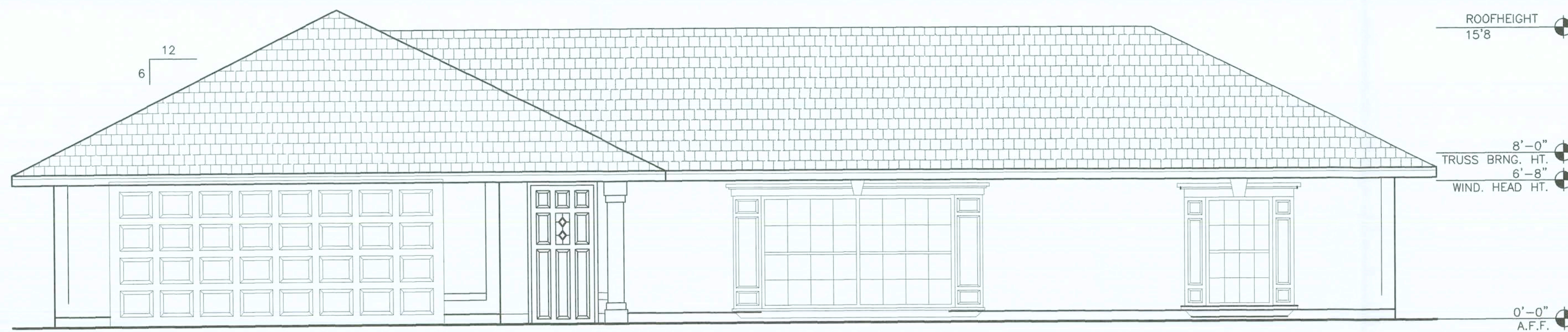
FRONT ELEVATION
