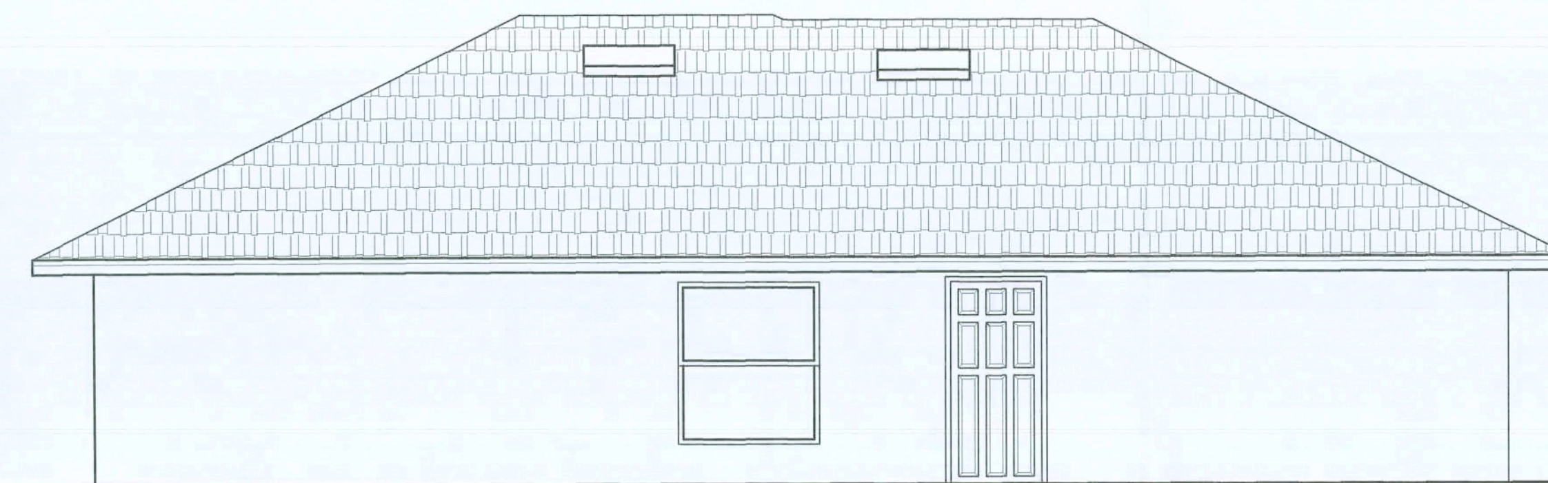
LEFT ELEVATION
