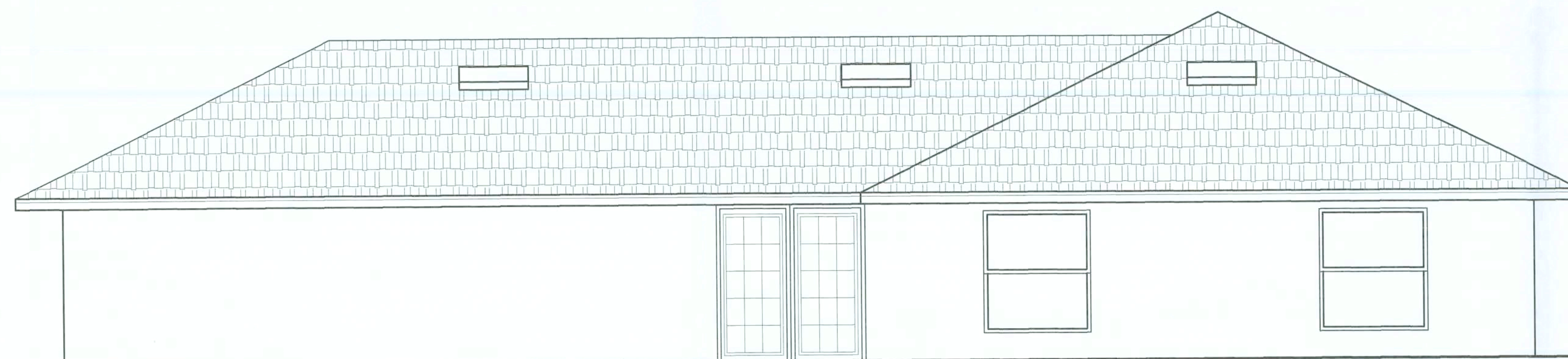
BACK ELEVATION
