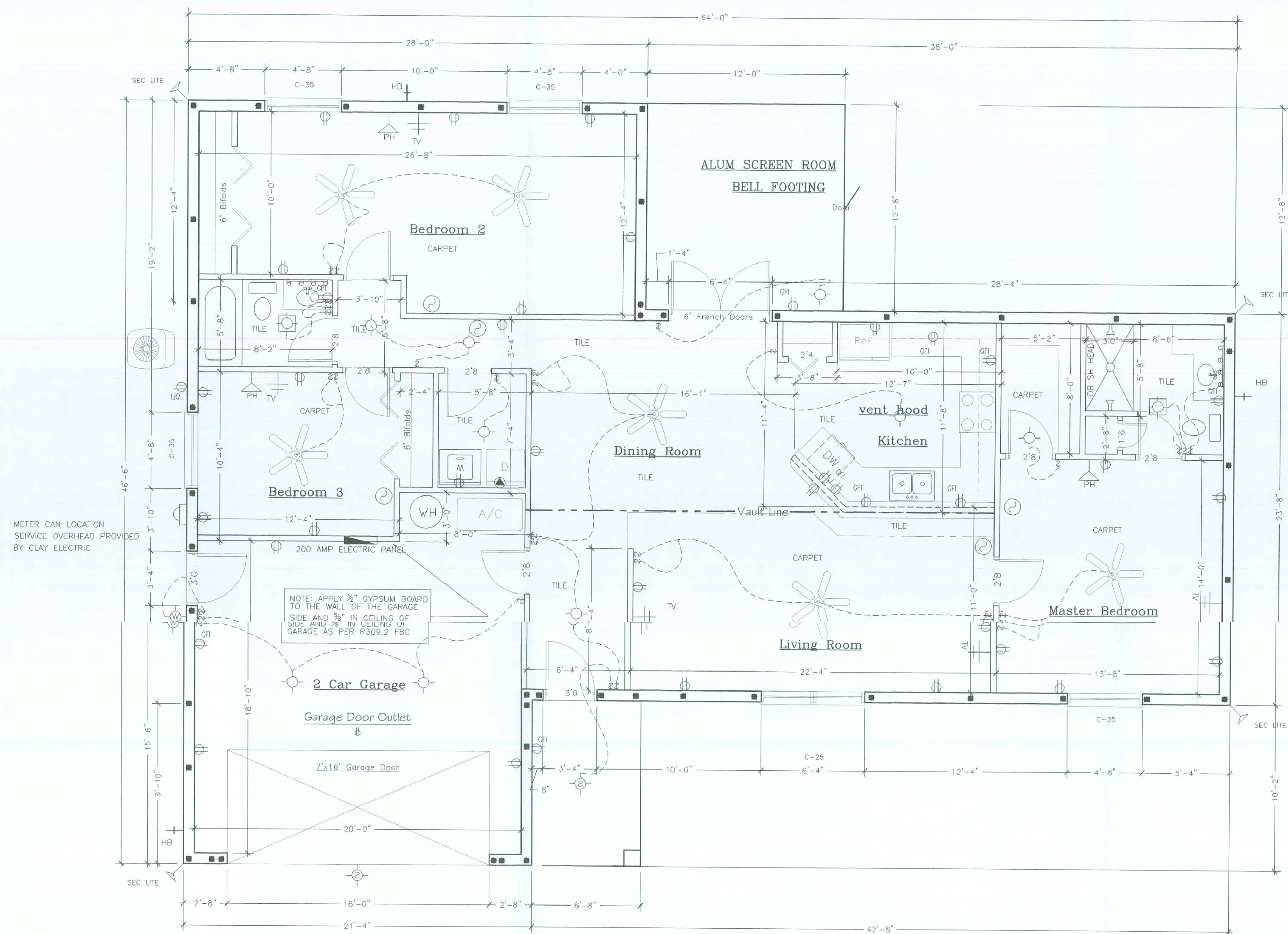
FLOOR PLAN
