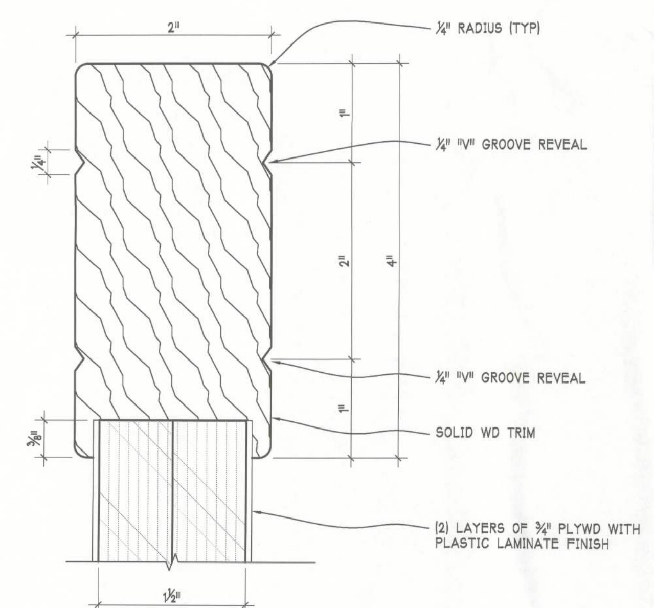
DIVIDER PANEL WD TRIM DETAIL FULL SCALE
