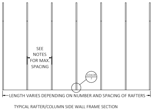
TYPICAL RAFTER/COLUMN SIDE WALL FRAME SECTION
