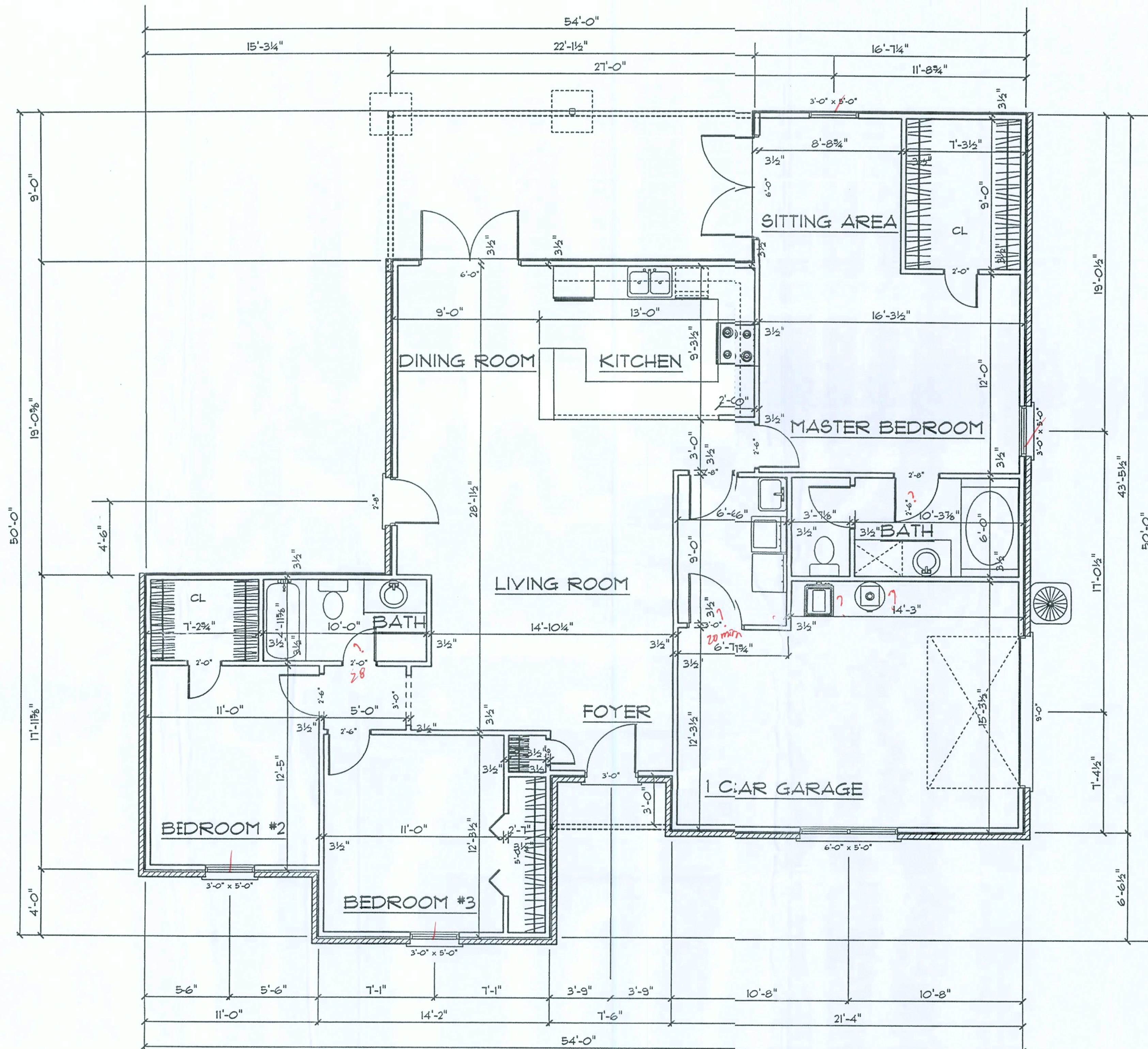
FLOOR PLAN
