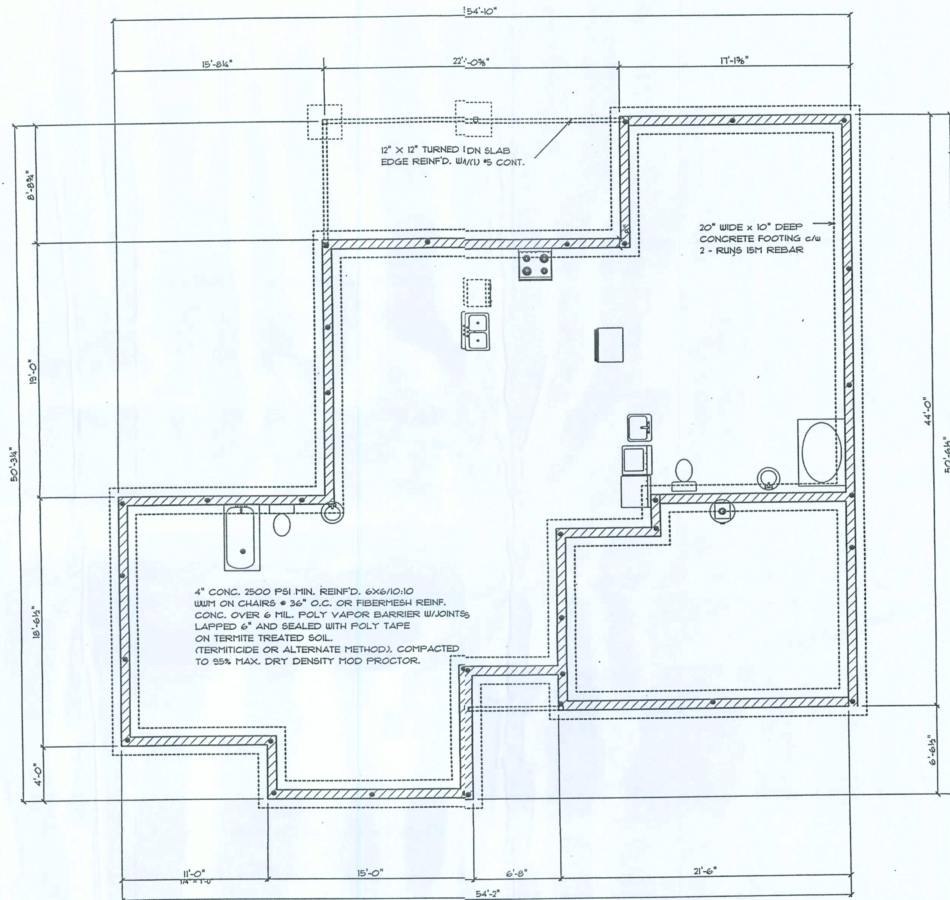
FOUNDATION PLAN
