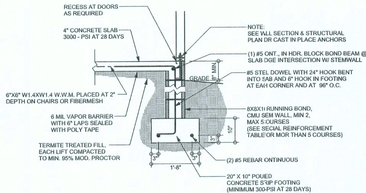
F6 S-2 TYPICAL NON - BEARING STEP FOOTING SCALE: 1/2" = 1'-0"
