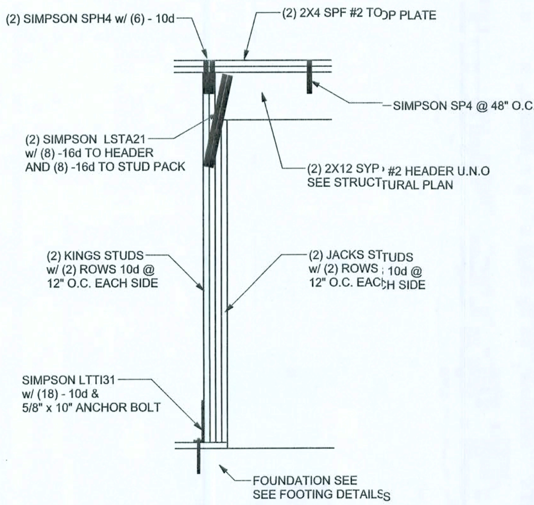
TYPICAL GARAGE DOOR HEADER STRAPPING DETAIL SCALE: 1/2" = 1'-0"
