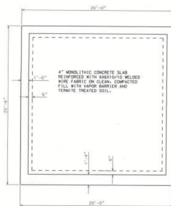
FOUNDATION PLAN
