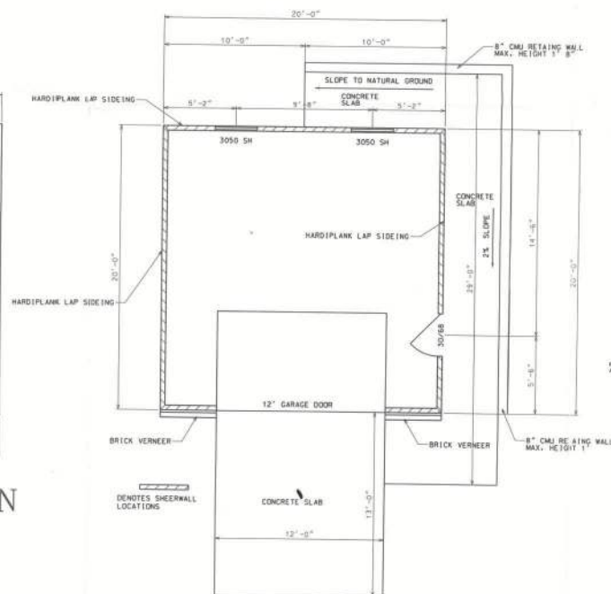
FLOOR PLAN
