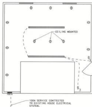
ELECTRICAL PLAN
