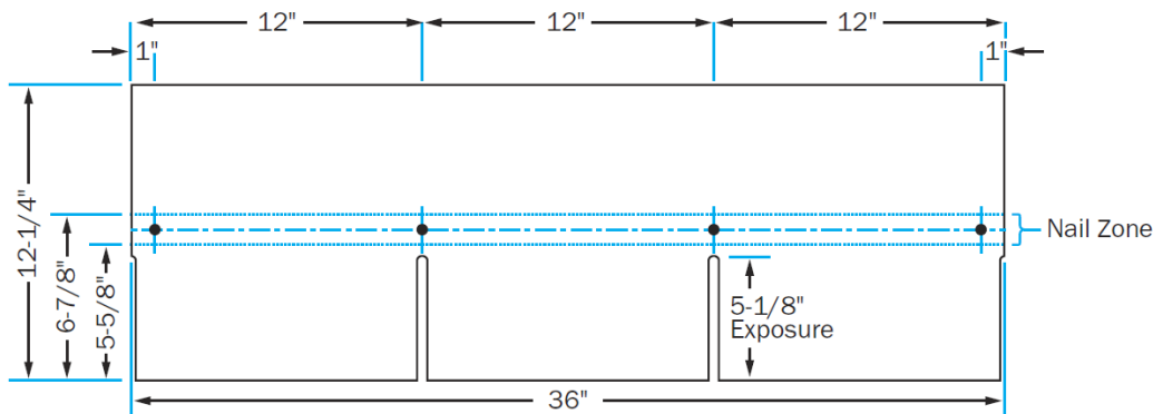
Figure 1. Elite Glass-Seal 4 Nail Pattern (Non-HVHZ only)
