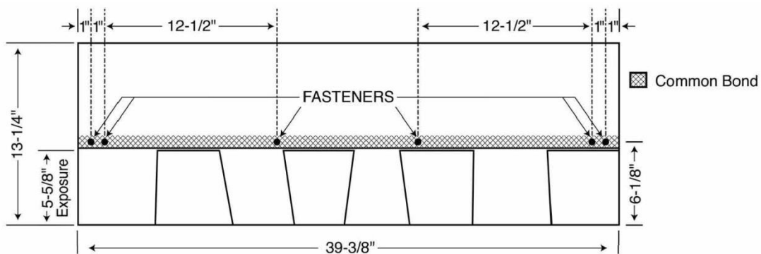
Figure 7. Heritage®, Heritage® Premium, & Heritage® Woodgate Alternate 6 Nail Pattern
