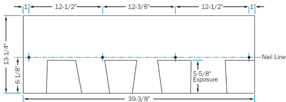
Figure 3. Heritage® & Heritage® Premium 4 Nail Pattern (non-HVHZ only)
