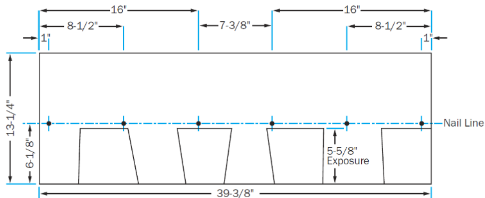
Figure 4. Heritage® & Heritage® Premium 6 Nail Pattern
