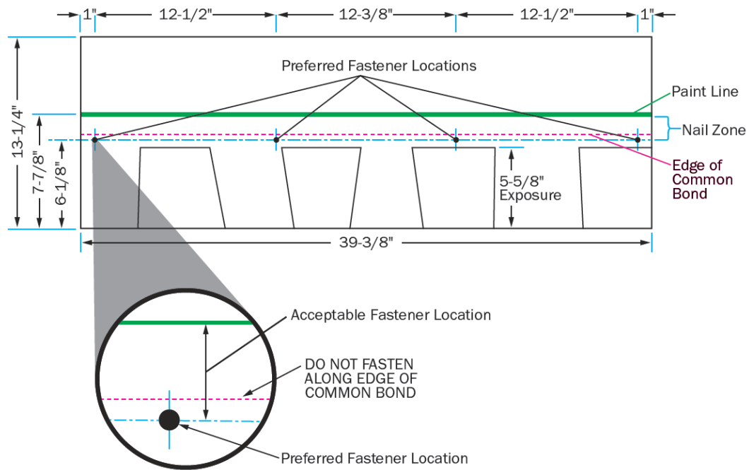
Figure 8. Heritage® (Tuscaloosa) Expanded Nail Zone
