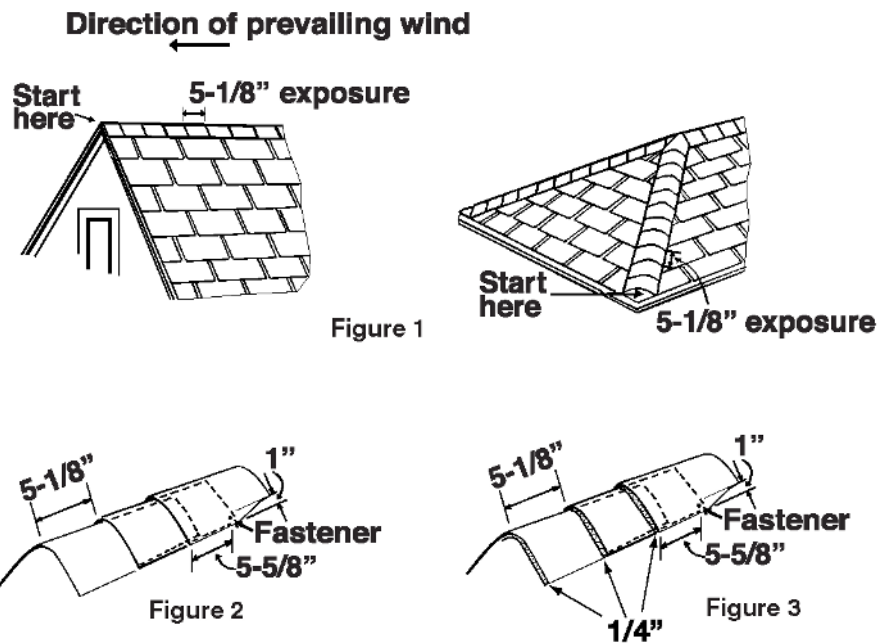
Figure 11. Hip & Ridge
