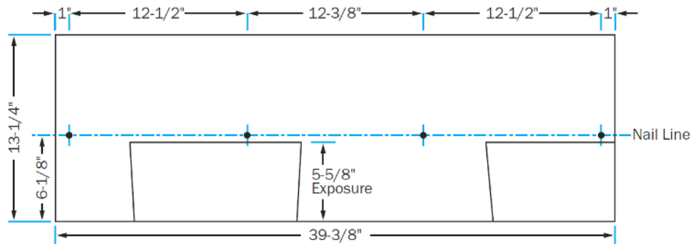
Figure 5. Heritage® Woodgate 4 Nail Pattern (non-HVHZ only)
