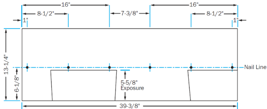
Figure 6. Heritage® Woodgate 6 Nail Pattern
