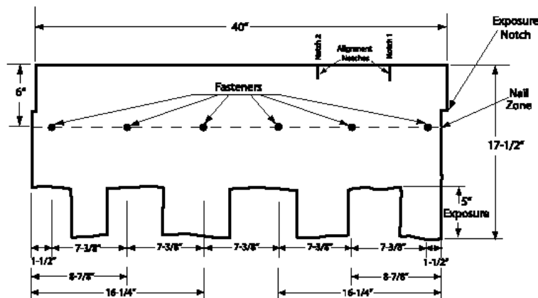
Figure 10. Heritage® Vintage® 6 Nail Pattern
