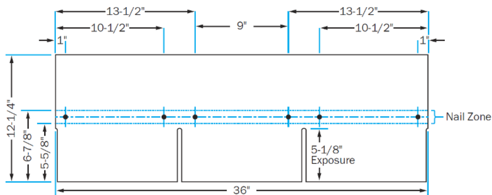
Figure 2. Elite Glass-Seal 6 Nail Pattern
