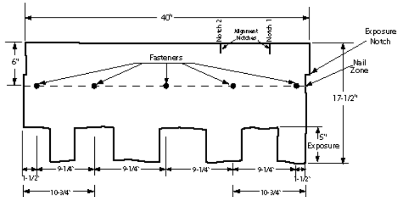
Figure 9. Heritage® Vintage® 5 Nail Pattern (non-HVHZ only)
