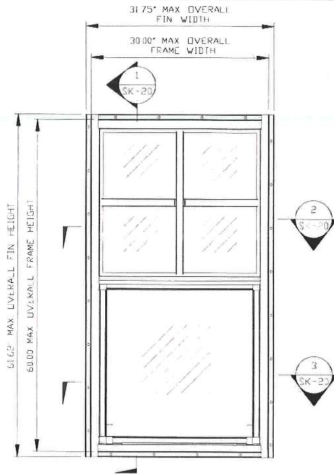
ELEVATION VIEW
