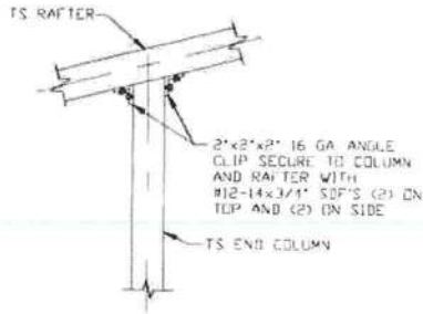
END COLUMN/RAFTER CONNECTION DETAIL
