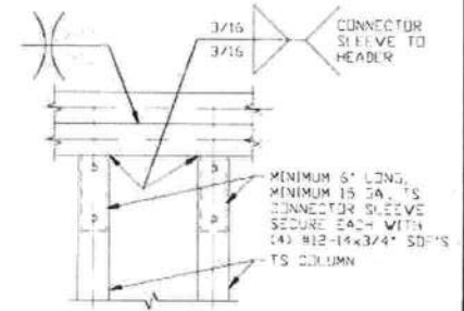
DOUBLE HEADER/COLUMN CONNECTION DETAIL
