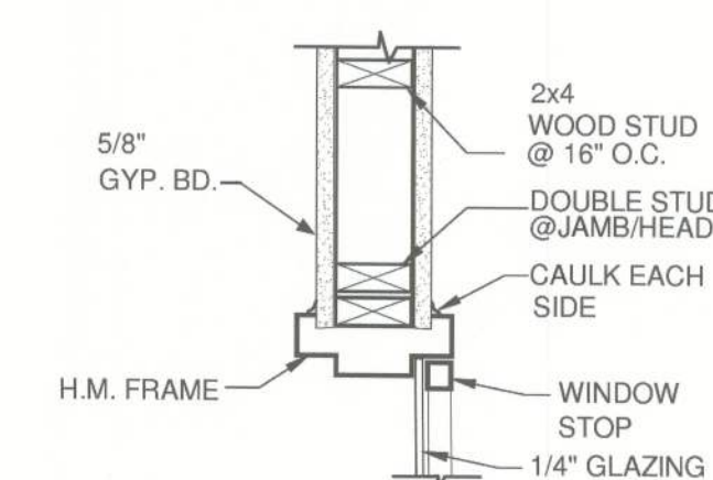
5 A1.6 INTERIOR HEAD JAMB / SILL DETAIL SCALE: 1 1/2" = 1'-0"
