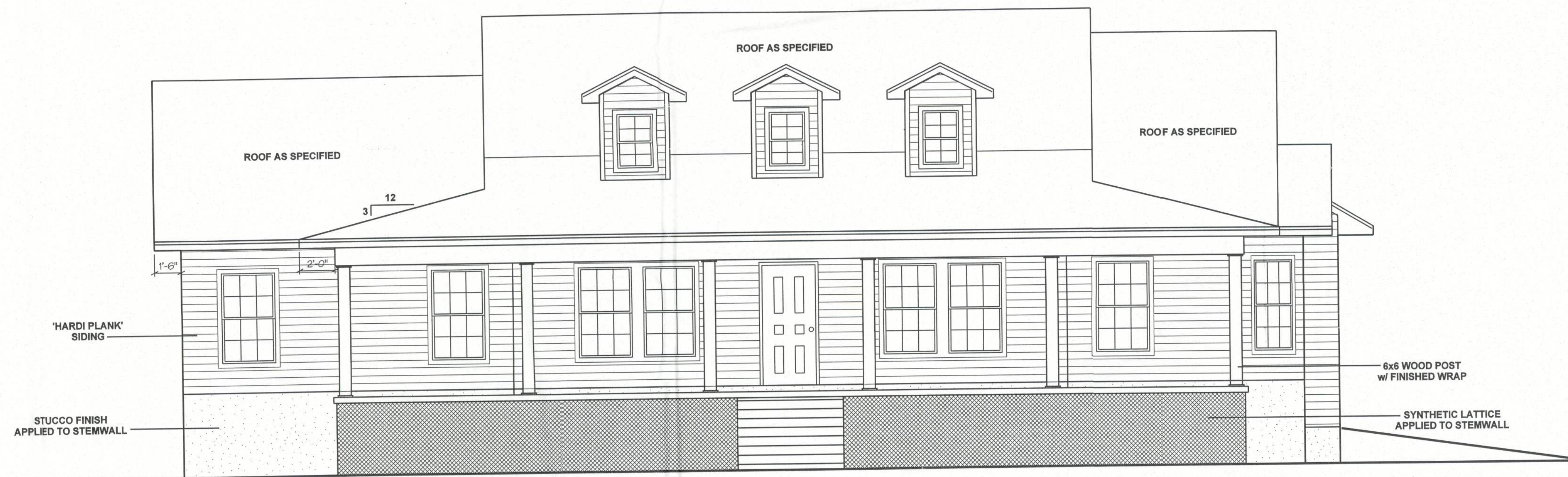
FRONT ELEVATION
