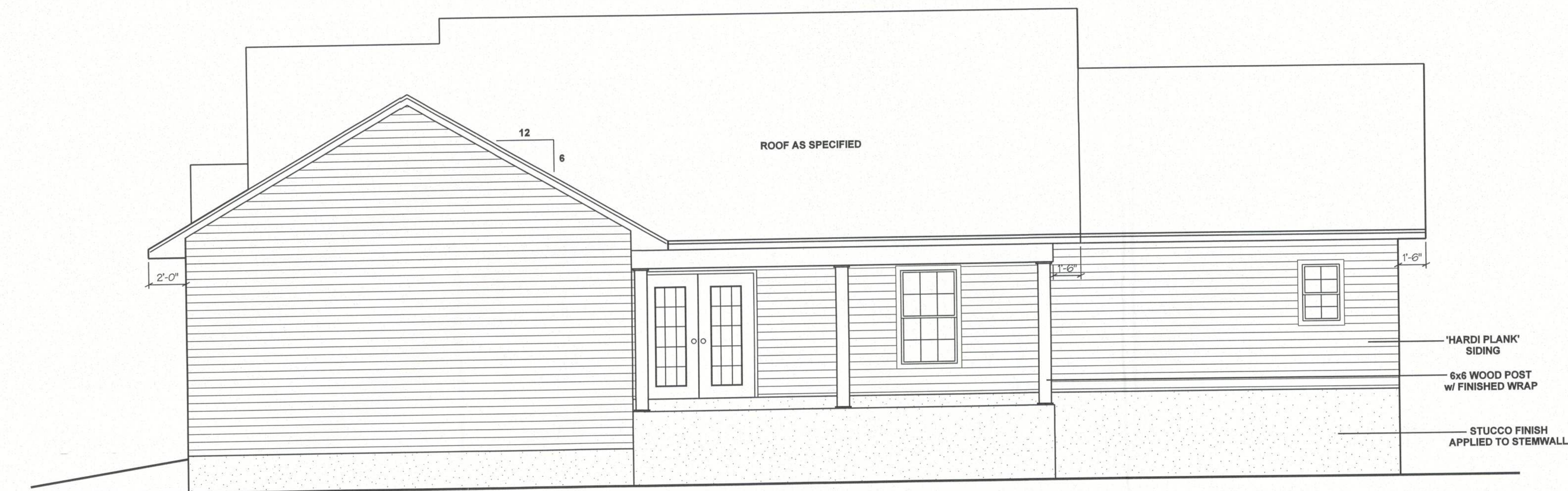
REAR ELEVATION
