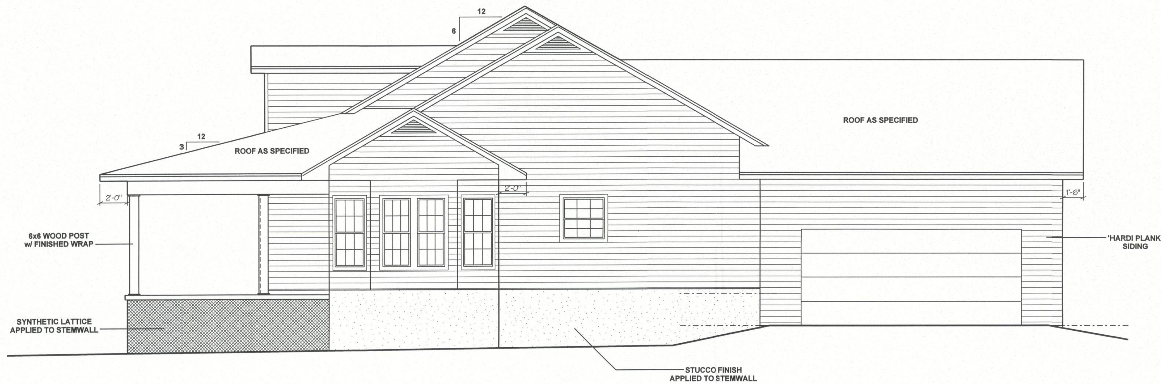
RIGHT SIDE ELEVATION
