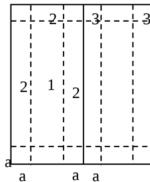
Figure 6-5 - External Pressure Coefficients, GCp
