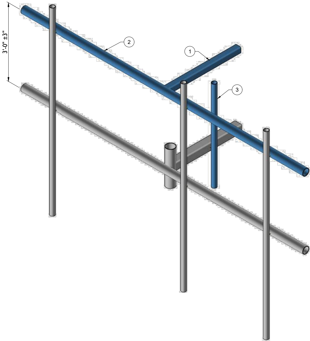
1 PROPOSED ISOMETRIC VIEW (TYP. ALL SECTORS)
