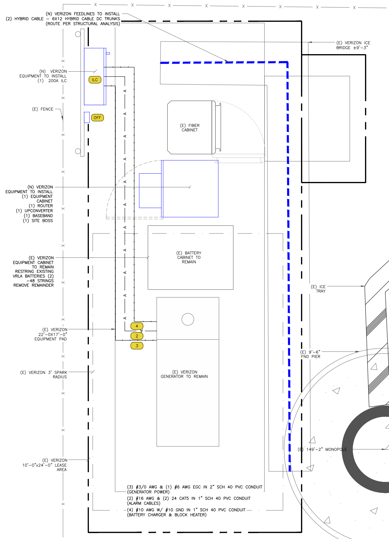
2 PROPOSED SITE PLAN SCALE: 1" = 6'-0" (FULL SIZE) 3/4"=1'-0" (11x17) 3/8"=1'-0" (11x17)
