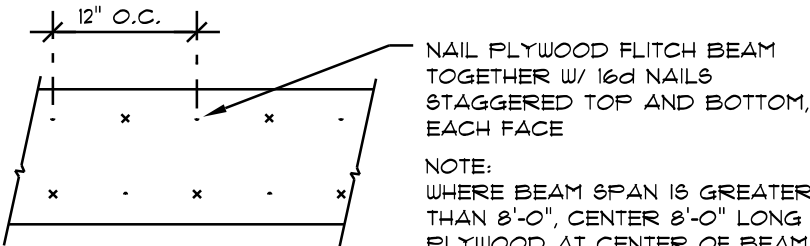
PLYWOOD FLITCH BEAM DETAIL NOT TO SCALE
