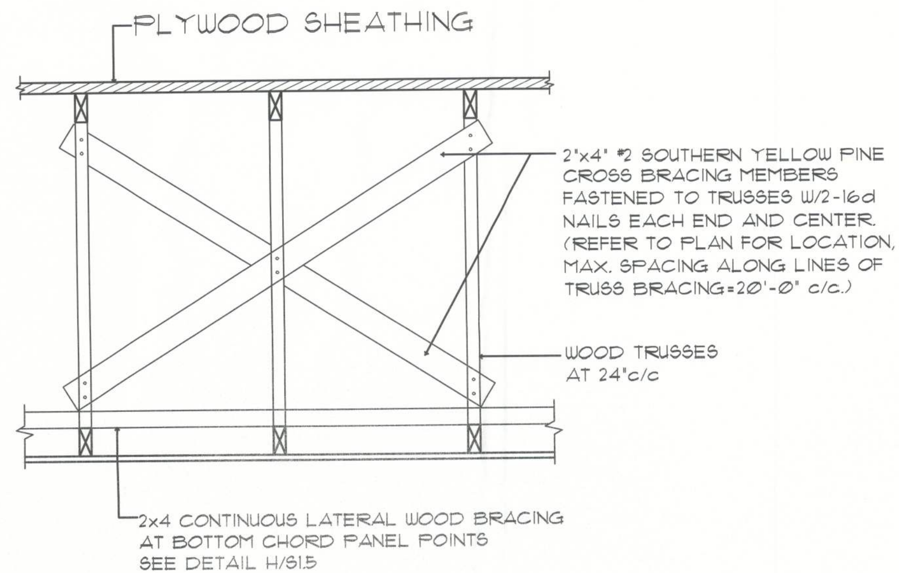
B TYPICAL TRUSS X-BRACING DETAIL
