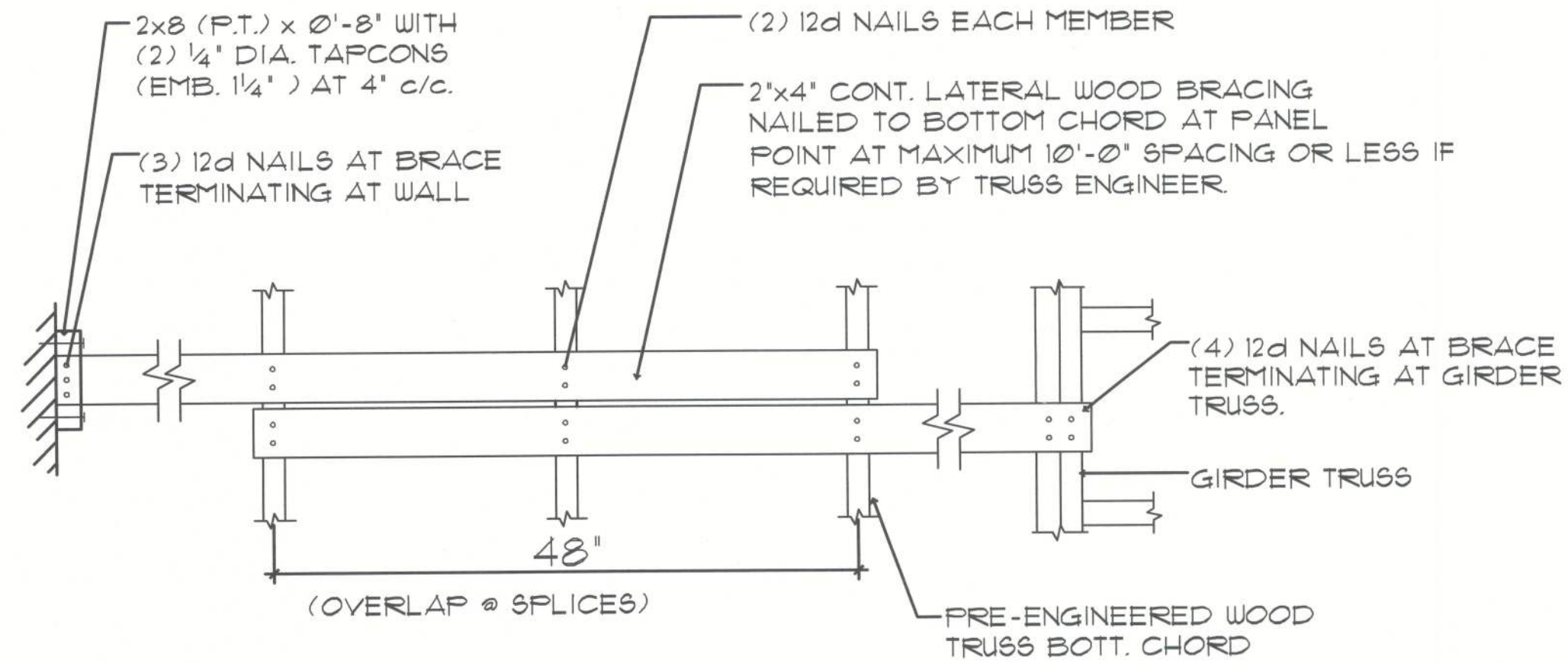
B CONTINUOUS LATERAL TRUSS BRACING DETAIL
