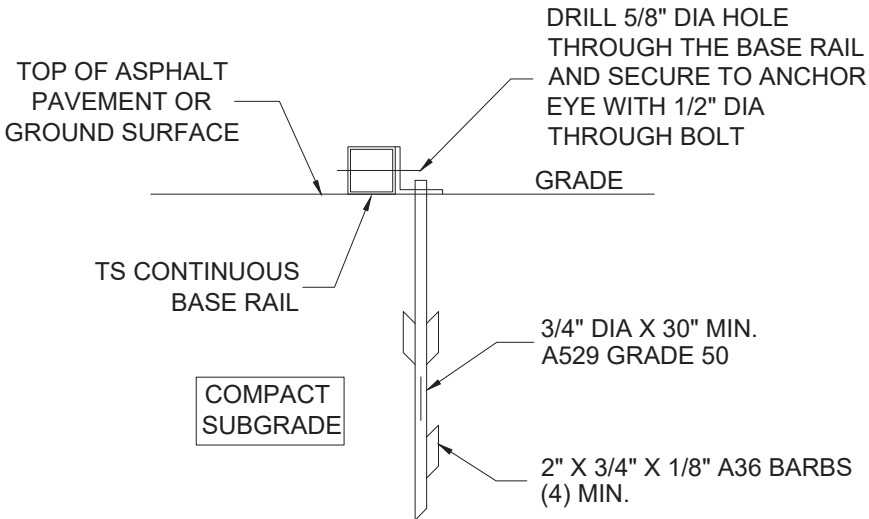
ASPHALT BASE ANCHORAGE (HP 9 BARBED DRIVE ANCHOR)
