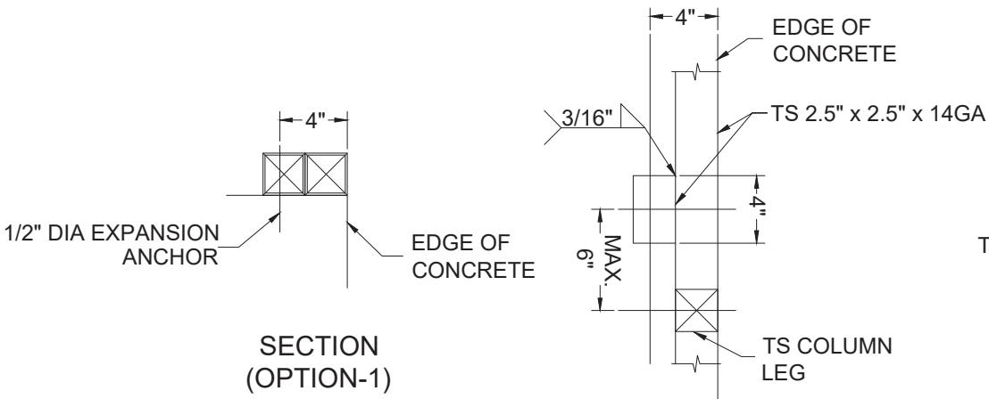
TYPICAL ANCHOR DETAIL WHEN BASE RAIL IS NEAR EDGE OF CONCRETE
