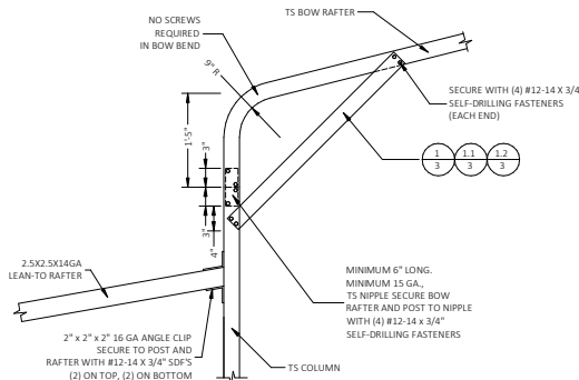
12" EXTENSION RAFTER/COLUMN DETAIL FOR EXTENSION RAFTER SPANS W < 12'-0" , IF THE KNEE BRACE ON THE OTHER END OF THE RAFTER IS PER DETAIL 1.2/3 FOR EXTENSION RAFTER SPANS W < 13'-0" , IF THE KNEE BRACE ON THE OTHER END OF THE RAFTER IS PER DETAIL 1.1/3 FOR EXTENSION RAFTER SPANS W < 15'-0" , IF THE KNEE BRACE ON THE OTHER END OF THE RAFTER IS PER DETAIL 1/3. SCALE: NTS
