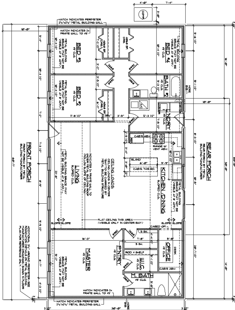
Floor Plan SCALE: 1/4" = 1'-0"
