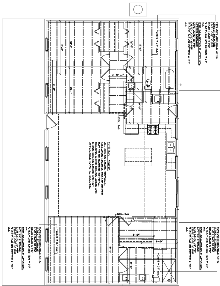
Ceiling Framing Plan SCALE: 1/4" = 1'-0"
