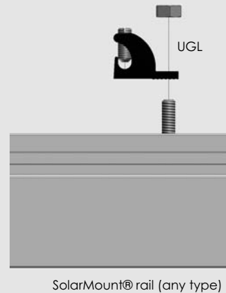
Figure 27. Slide 1/4-inch hex bolt into top mounting slot of any SolarMount® rail (standard, HD, or light). Secure nut with 7/16-inch crescent wrench with sufficient torque for lug serrations to penetrate anodized surface of rail.
