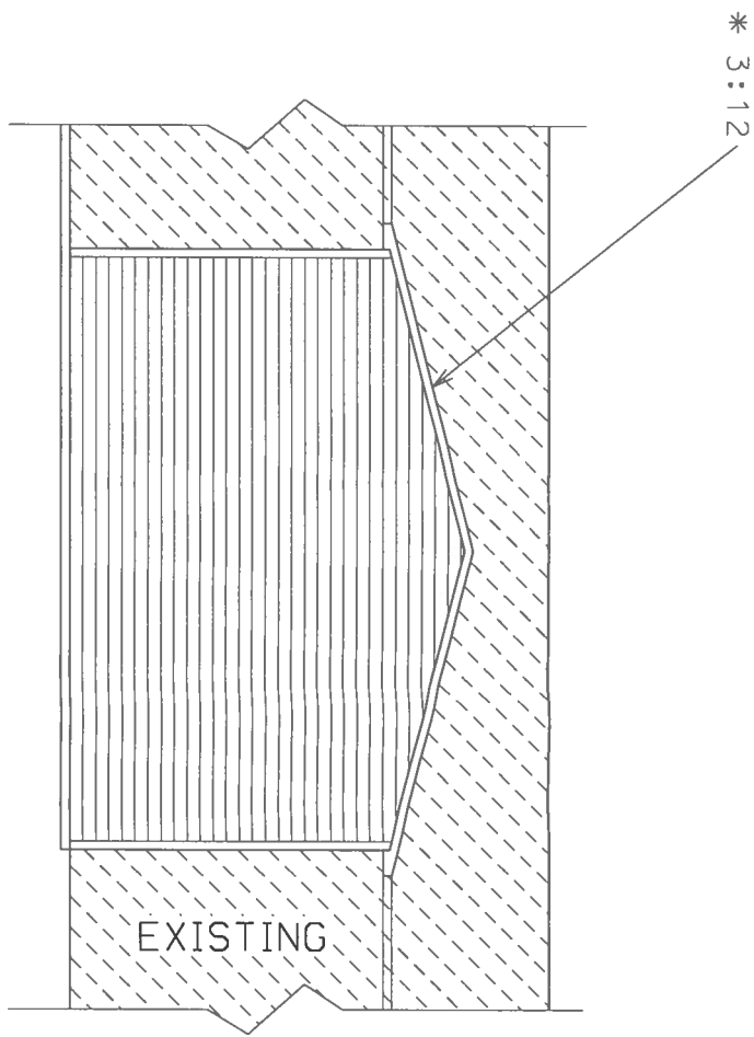
MODEL 2 - FRONT ELEVATION 0 4' 8' scale
