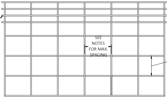
TYPICAL SIDE ELEVATION - VERTICAL ROOF/SIDING OPTION
