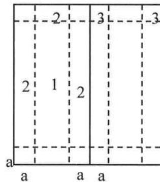
Figure 6-5 - External Pressure Coefficients, GC_p Loads on Components and Cladding for Buildings w/ H_t \leq 60 ft
