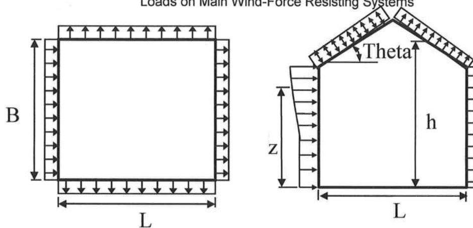
Figure 6-3 - External Pressure Coefficients, Cp
