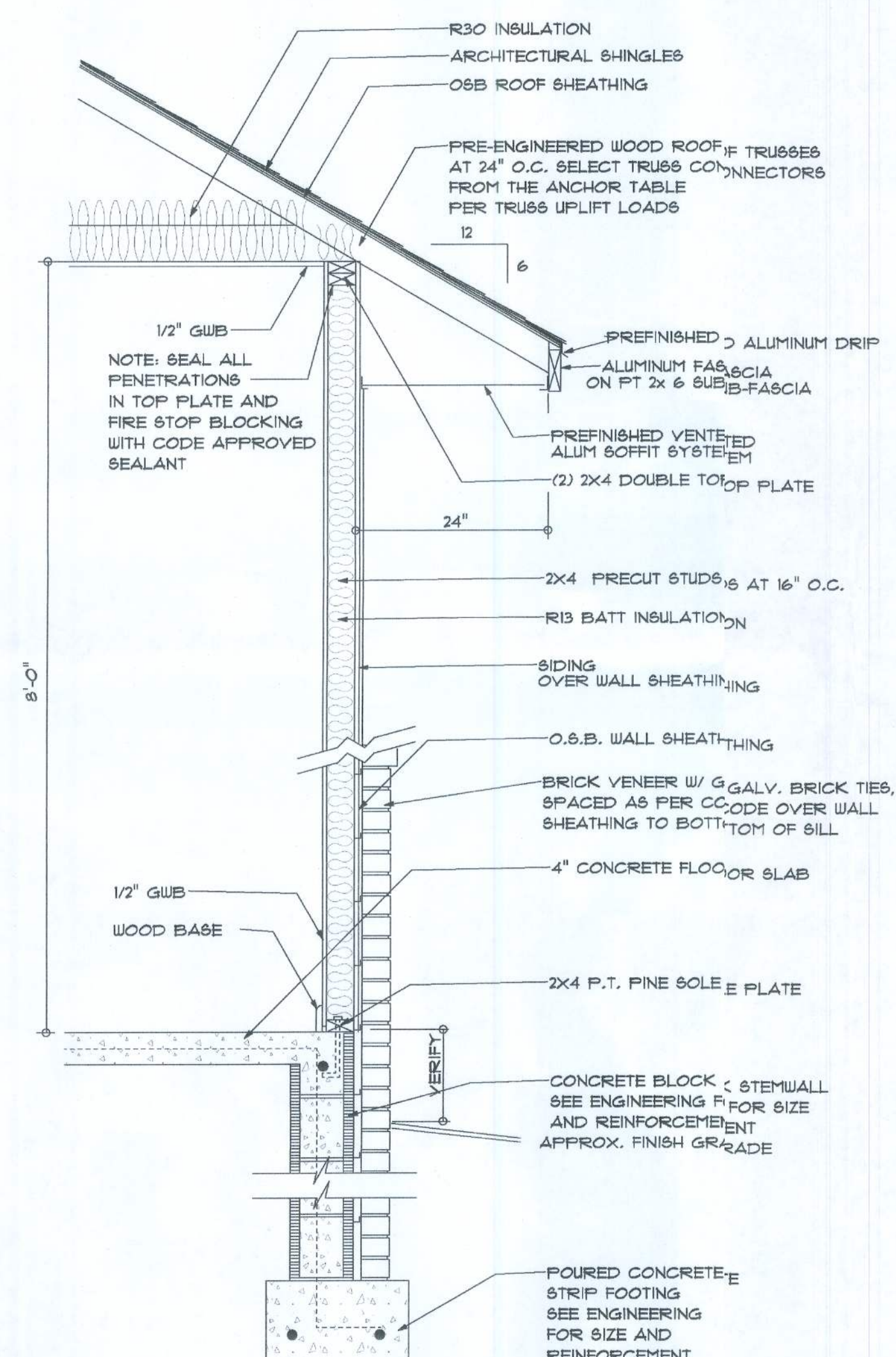
TYPICAL DESIGN WALL SECTION NON - STRUCTURAL DATA
