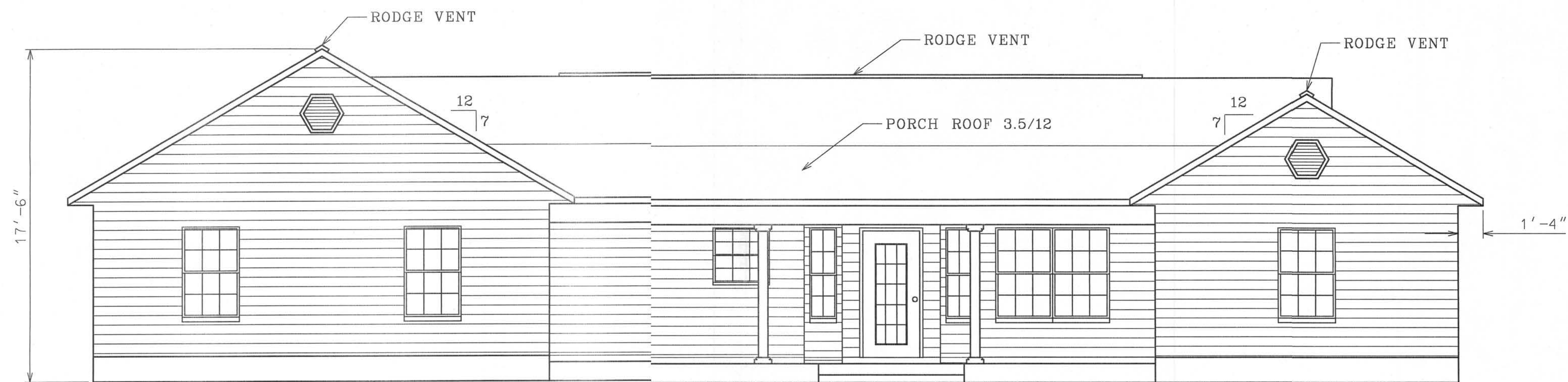
REAR ELEVATION
