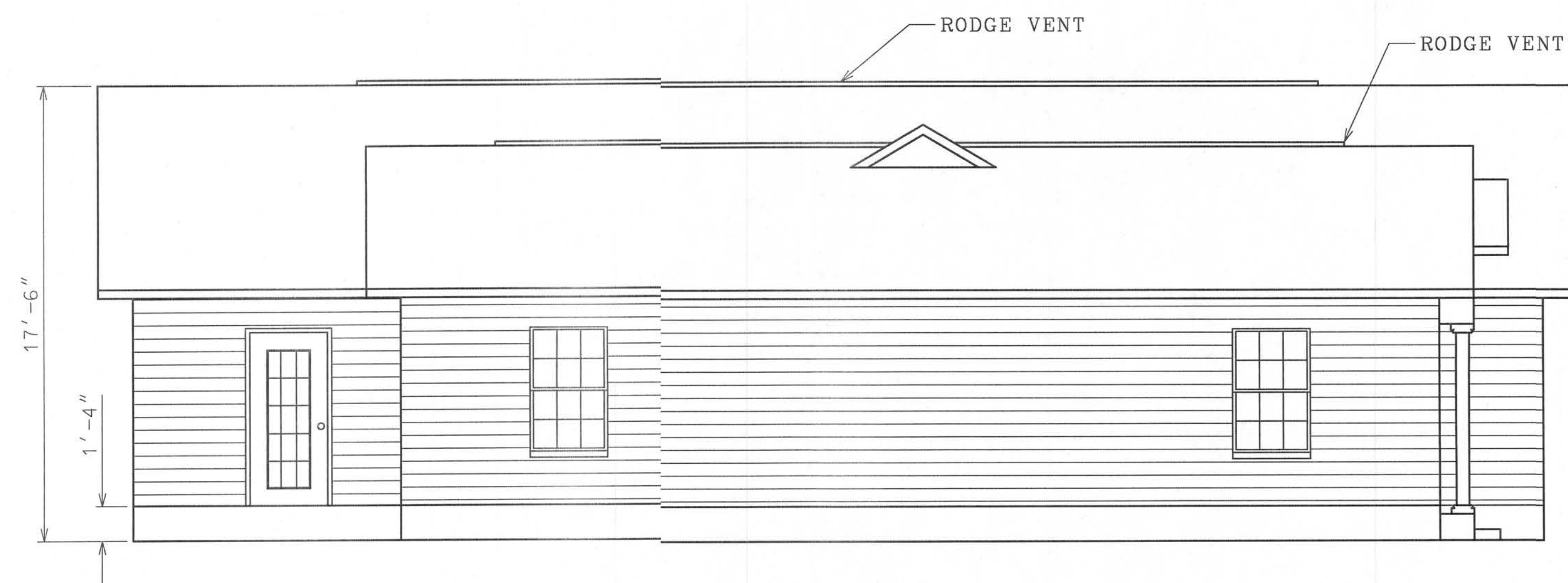
LEFT ELEVATION
