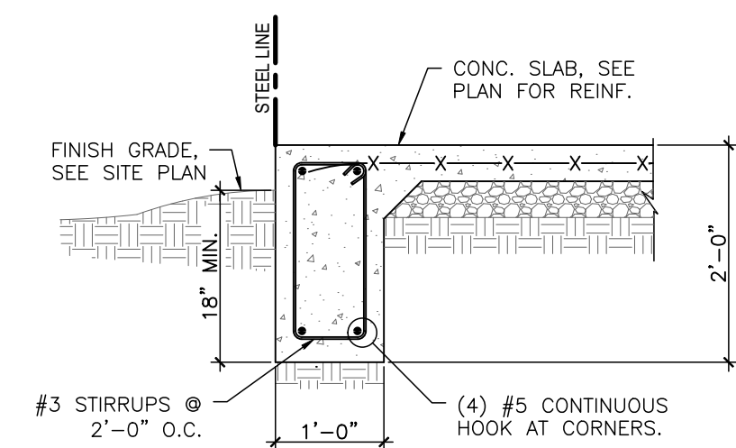
S1 PERIMETER FOOTING
