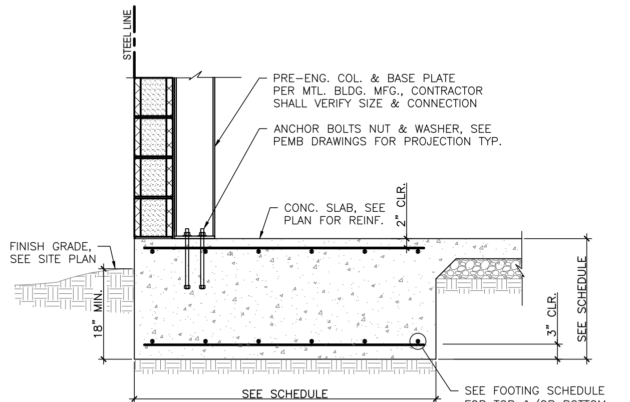
S4 FOOTING SECTION
