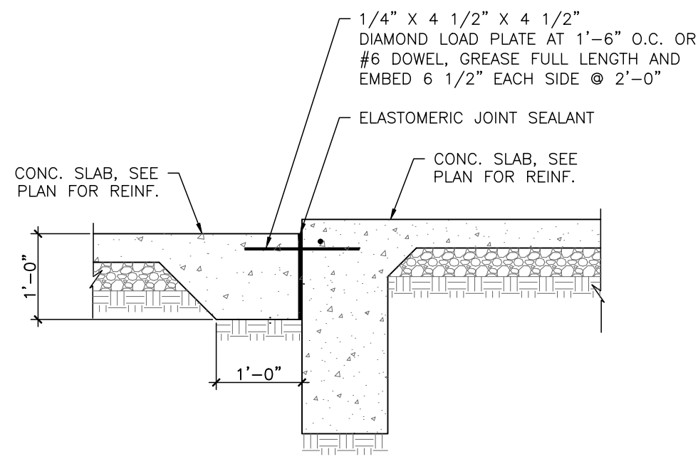
S5 PERIMETER FOOTING
