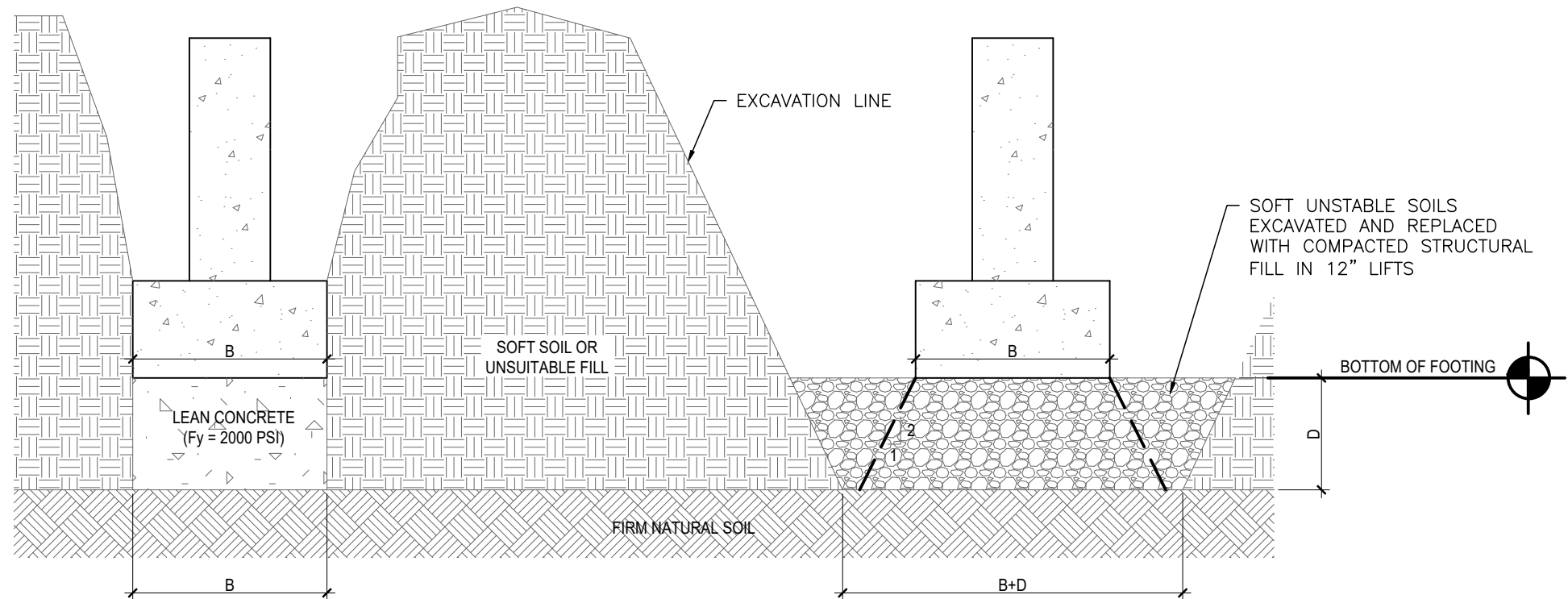
UNDERCUT EXCAVATION FOR UNSTABLE SOILS
