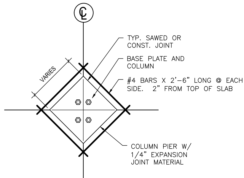
TYPICAL COLUMN ISOLATION
