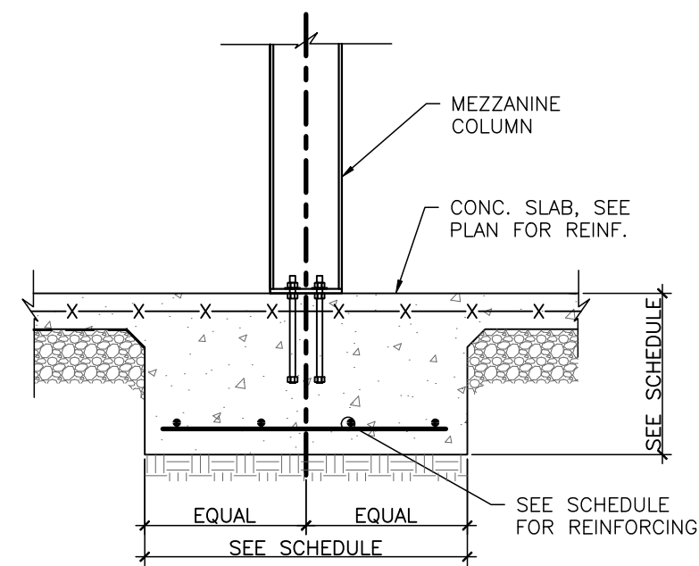
S3 TYPICAL INTERIOR FOOTING
