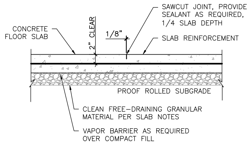
TYPICAL CONTROL JOINTS
