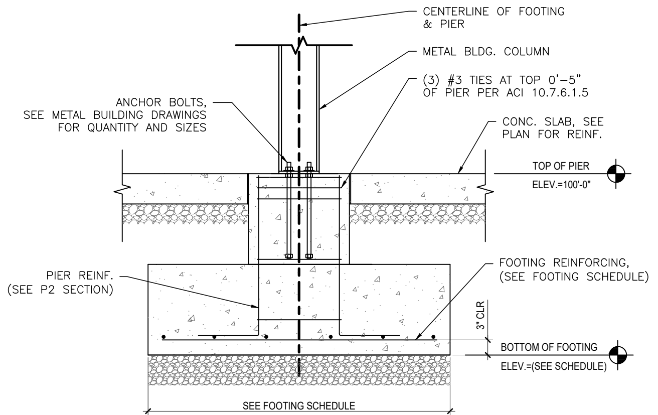
FOOTING SECTION
