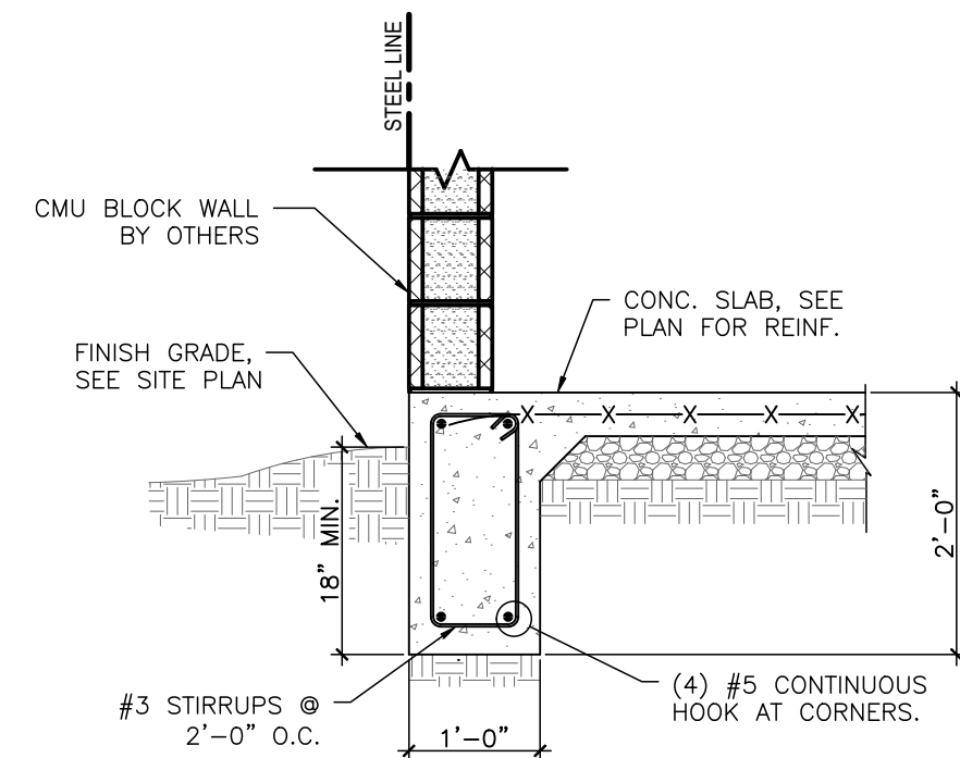
S2 PERIMETER FOOTING
