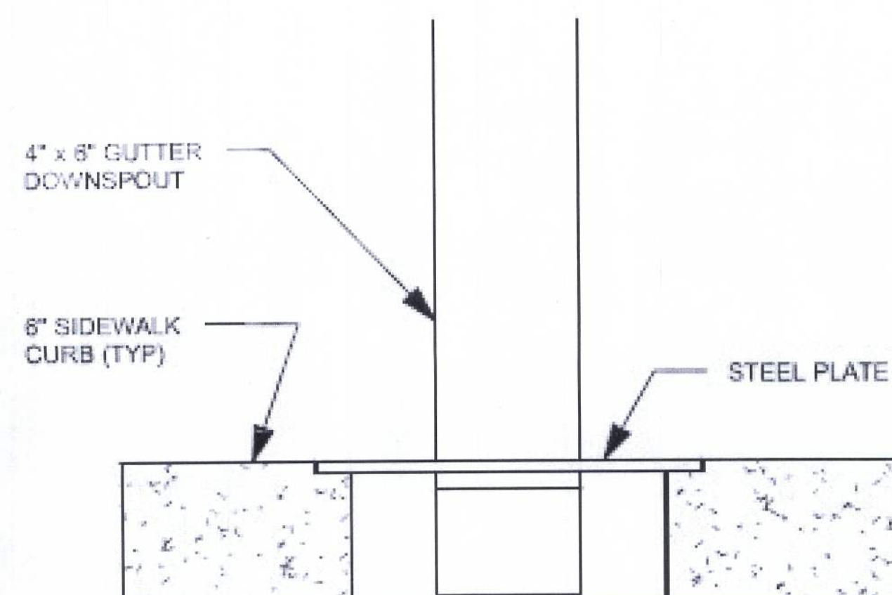
GUTTER DOWNSPOUT DETAIL AT SIDEWALK N.T.S.
