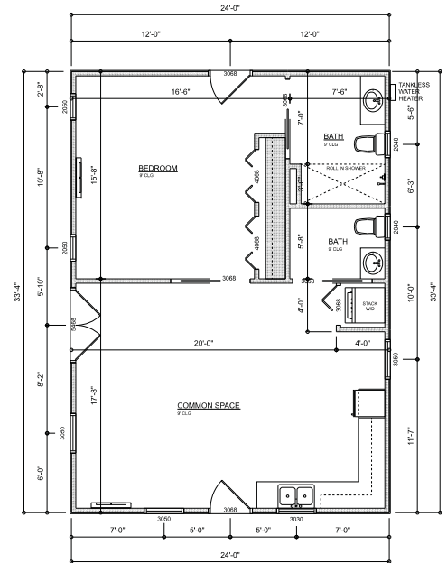
DIMENSIONED FLOOR PLAN SCALE: 1/4" = 1'-0"
