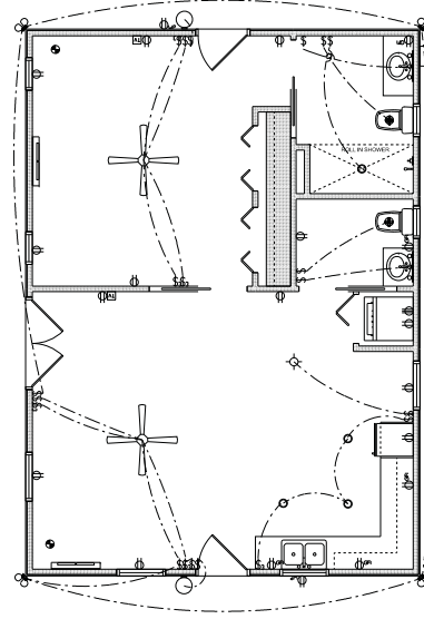
ELECTRICAL FLOOR PLAN SCALE: 1/4" = 1'-0"
