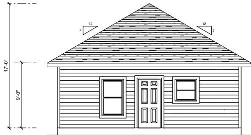
FRONT ELEVATION SCALE: 1/4" = 1'-0"
