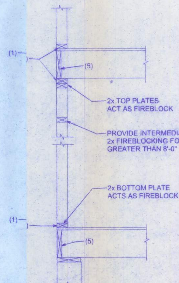
PLATFORM FRAMING
