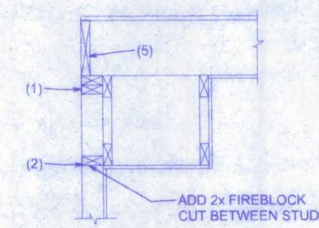
SOFFIT/DROPPED CLG.
