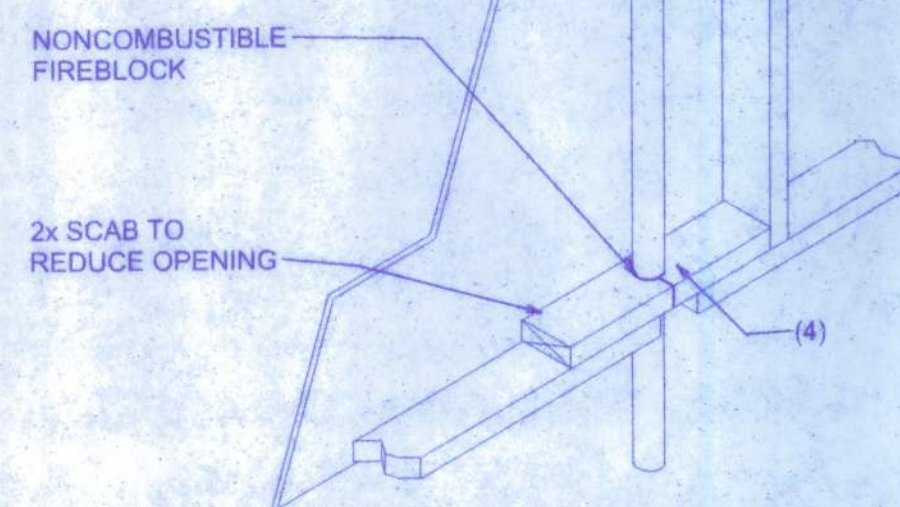
PENETRATIONS
