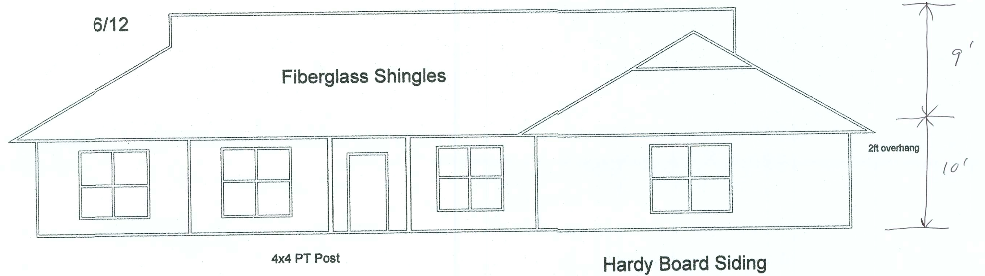
Front Elevation
