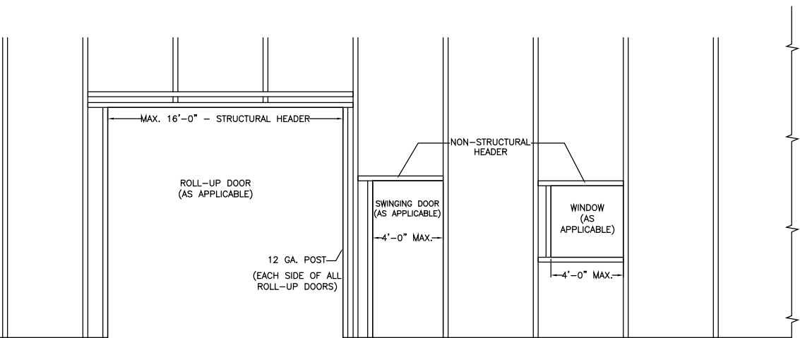
TYPICAL SIDE WALL ELEVATION
