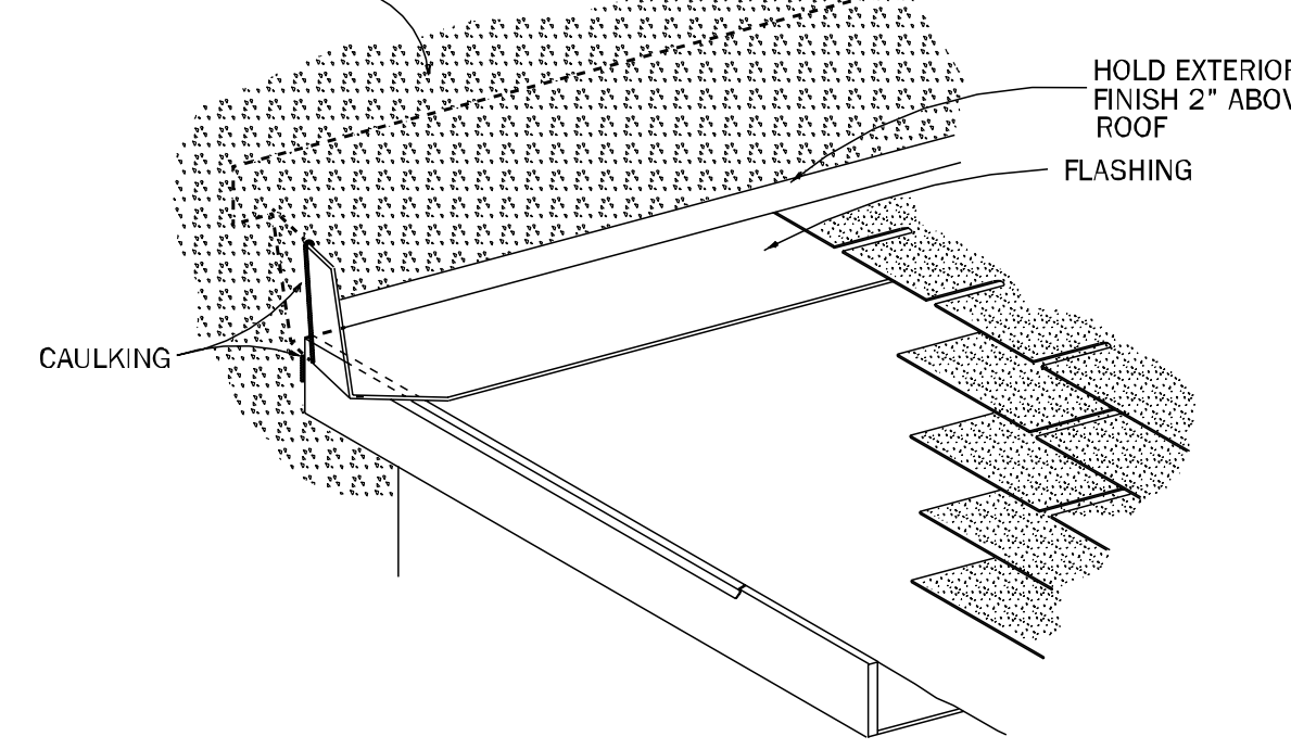
FLASHING INSTALLATION WHERE ROOF MEETS VERTICAL WALL
