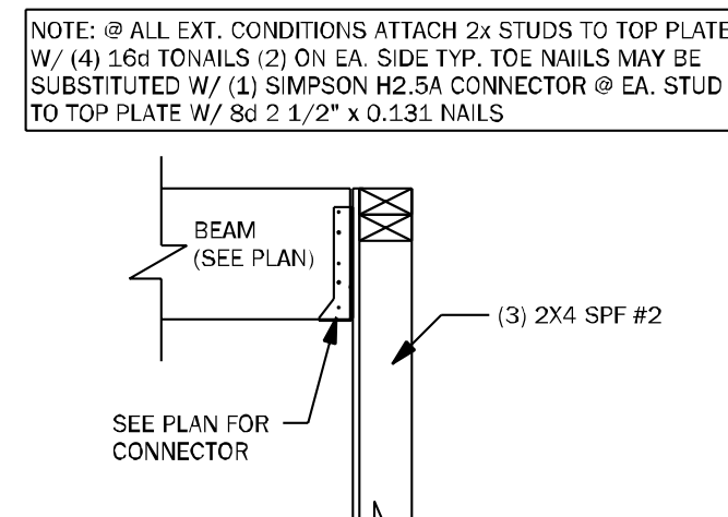
CD25 BEAM TO WALL CONNECTION N.T.S.
