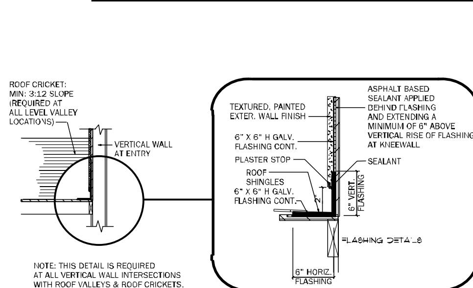
FIGURE 3: CORNER DETAIL
