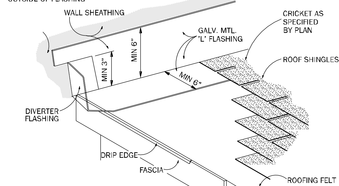
FIGURE 2: WALL FINISH
