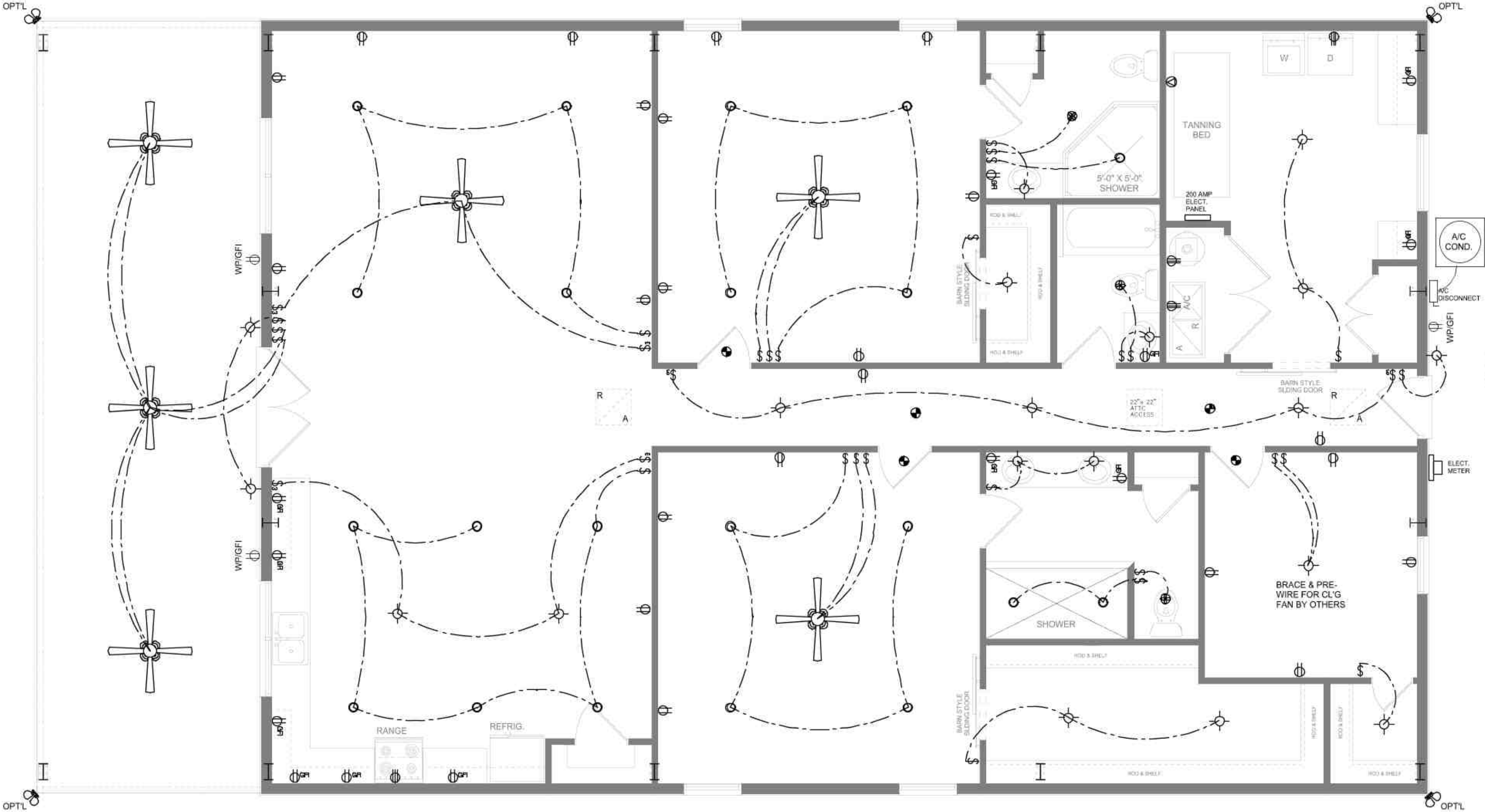
ELECTRICAL PLAN SCALE: 1/4" = 1'-0"
