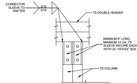
9B DOUBLE HEADER/COLUMN CONNECTION SCALE : N.T.S.
