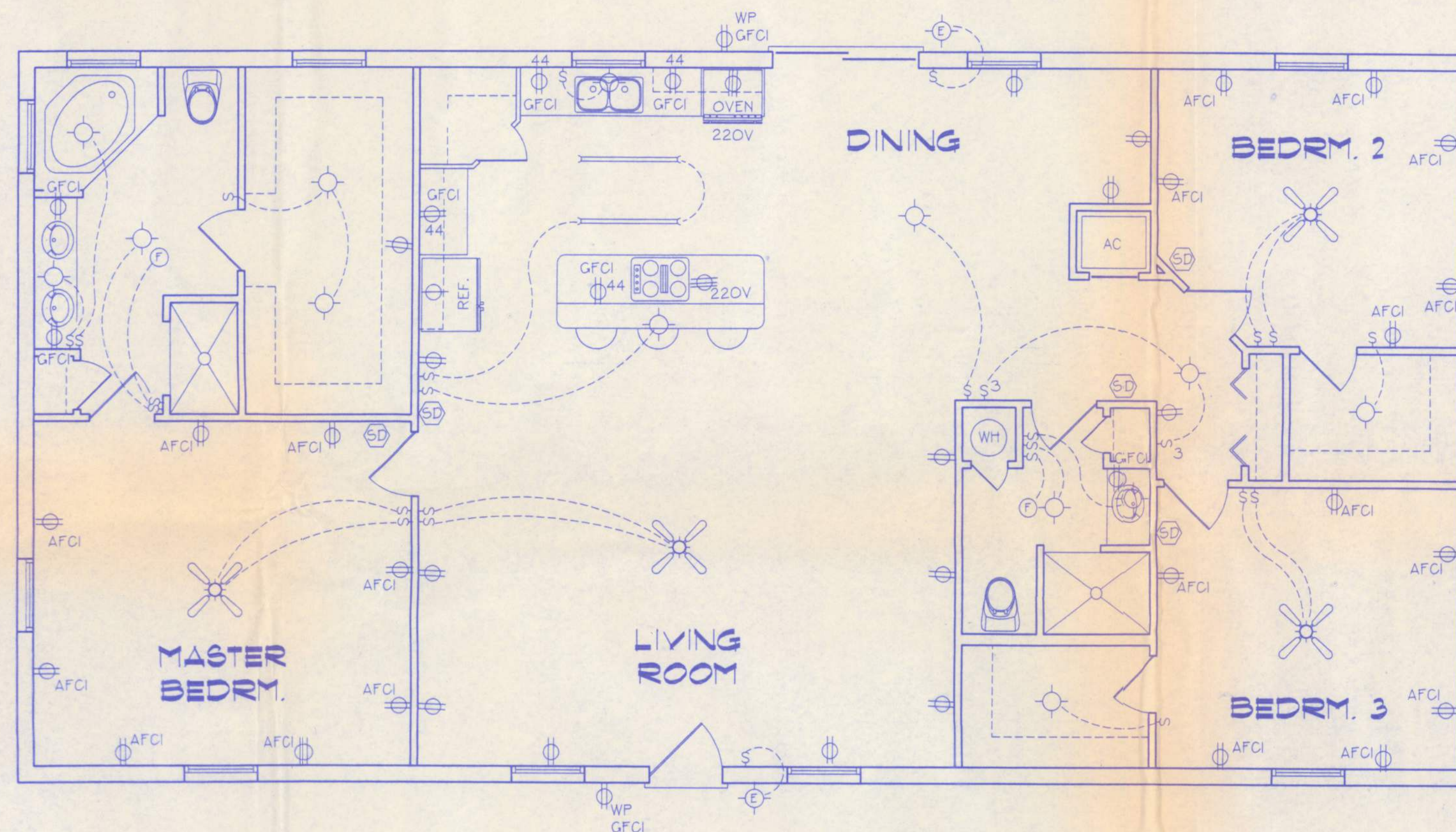
ELECTRICAL PLAN NOT TO SCALE
