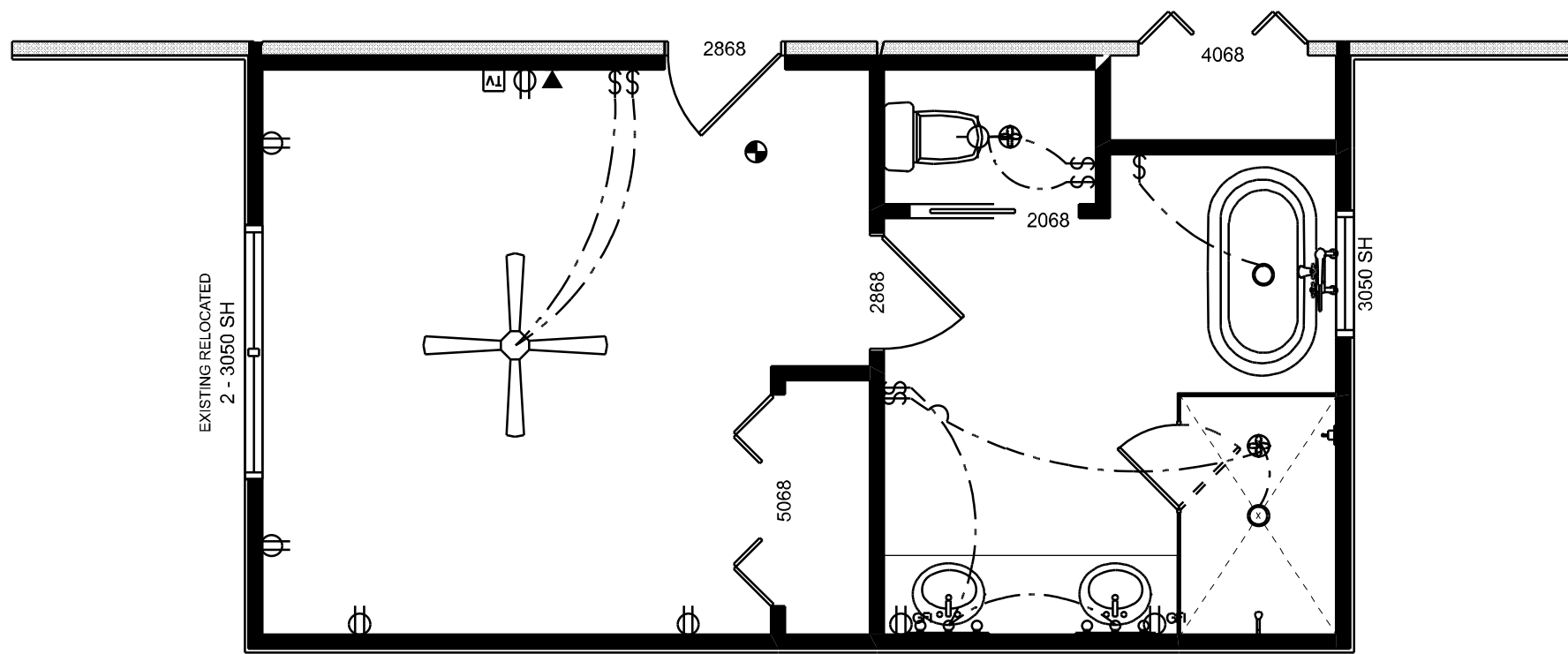
ELECTRICAL PLAN SCALE: 1/4" = 1'-0"
