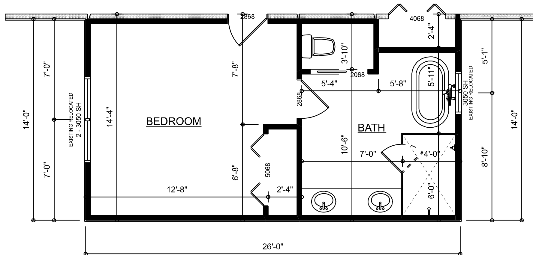
ADDITION FLOOR PLAN SCALE: 1/4" = 1'-0"
