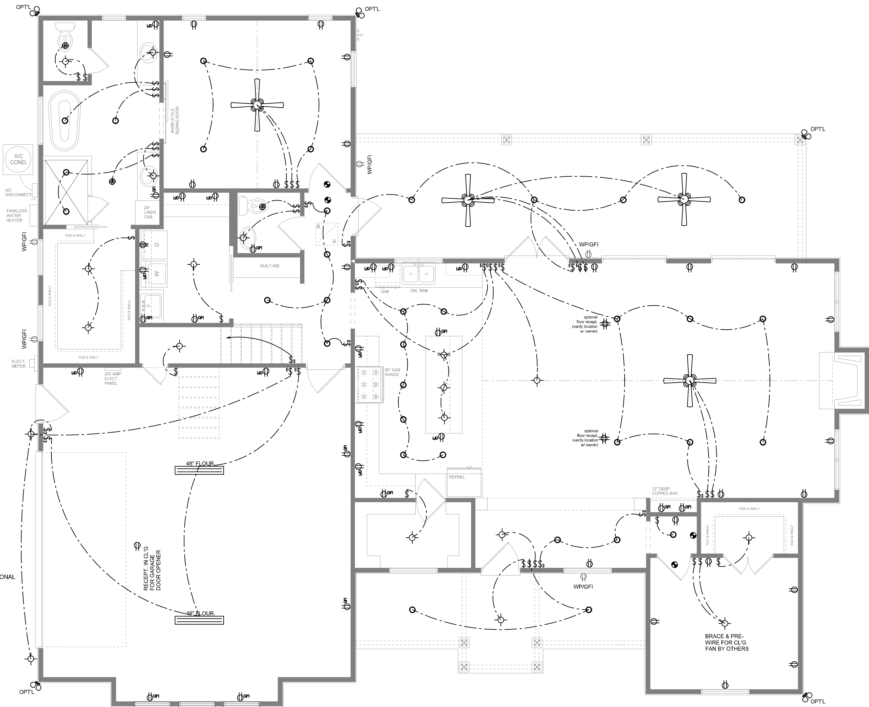
MAIN FLOOR ELECTRICAL SCALE: 1/4" = 1'-0"
