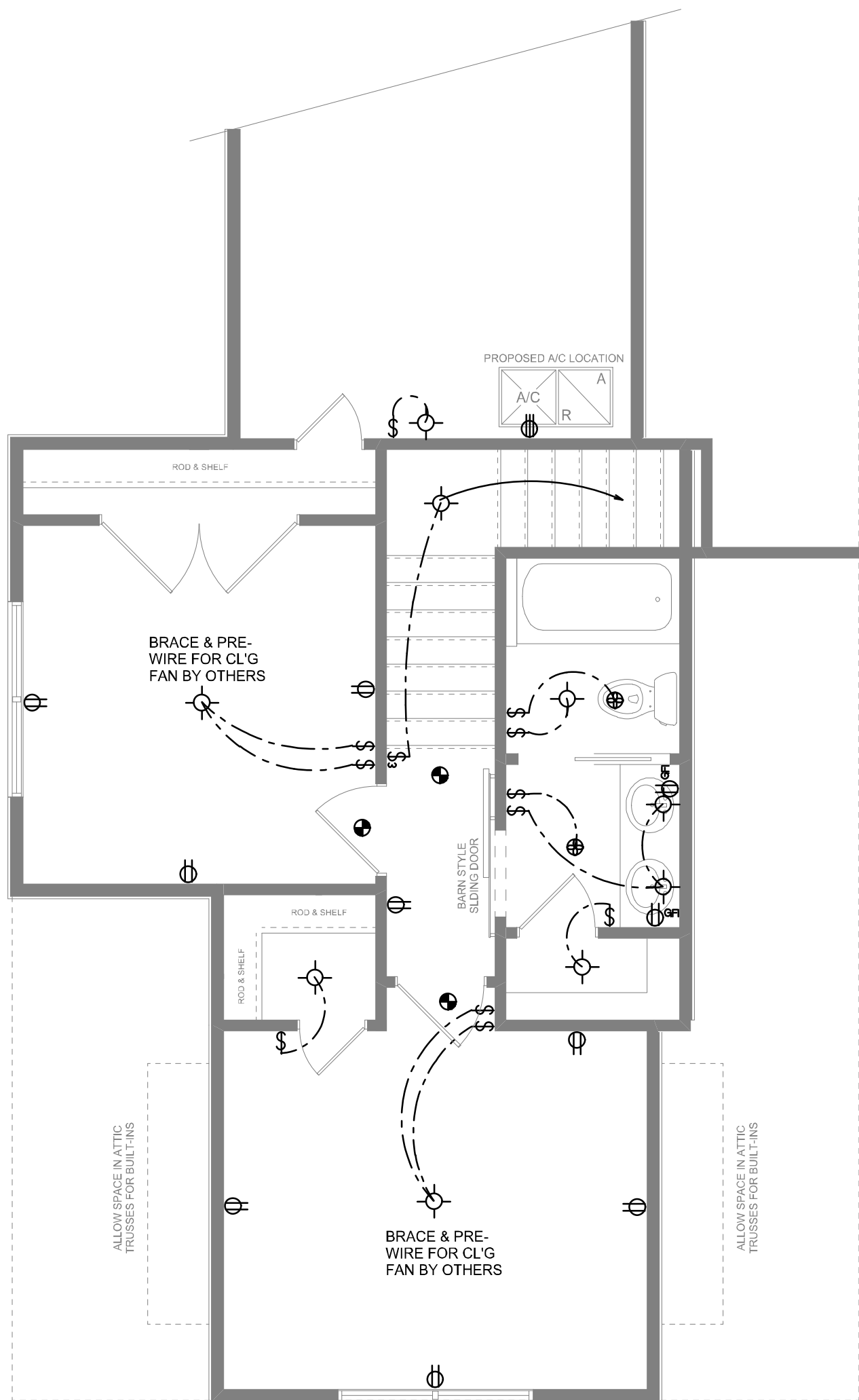
2ND FLOOR ELECTRICAL SCALE: 1/4" = 1'-0"
