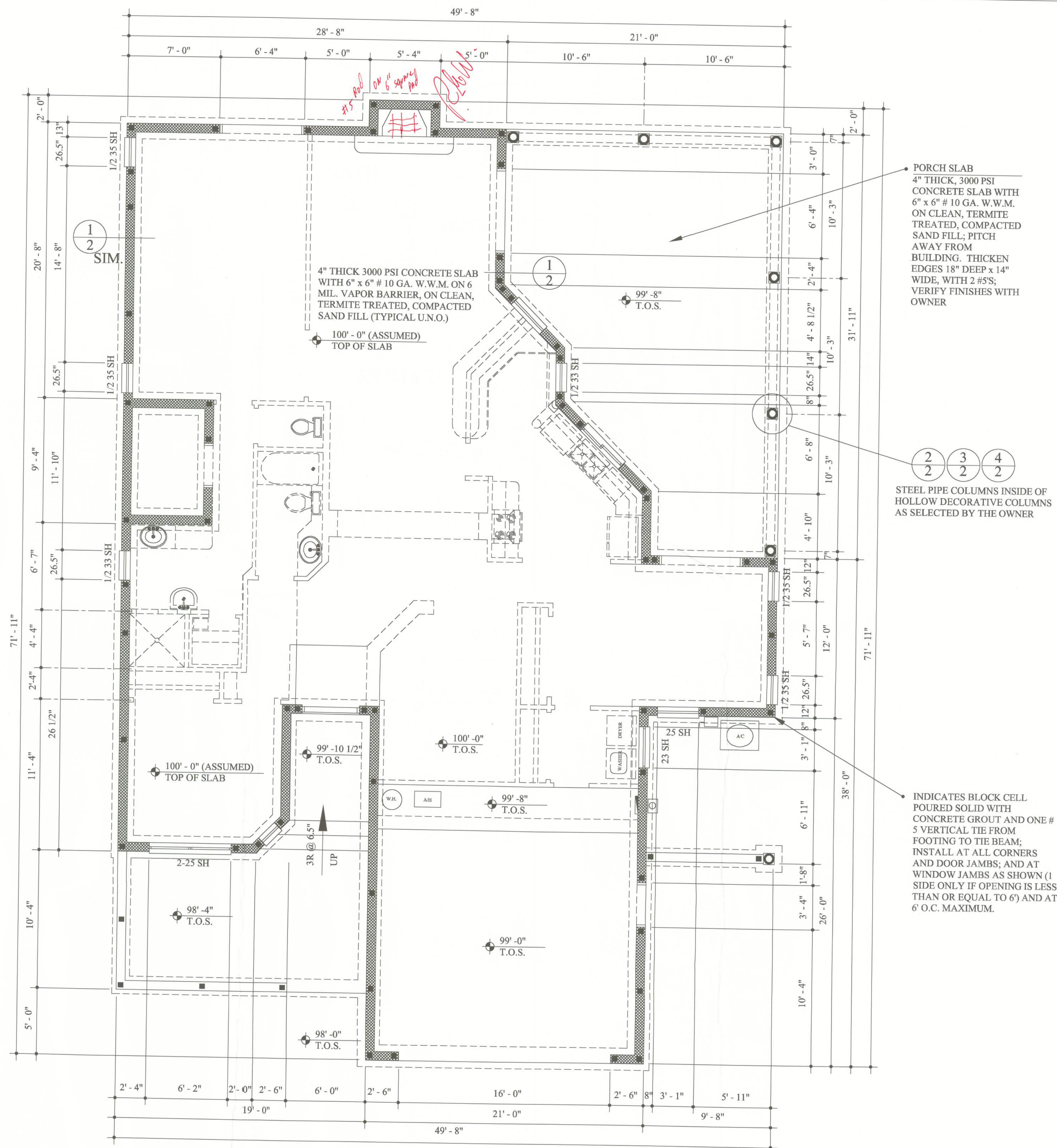
FOUNDATION PLAN 1/4" = 1' - 0"
