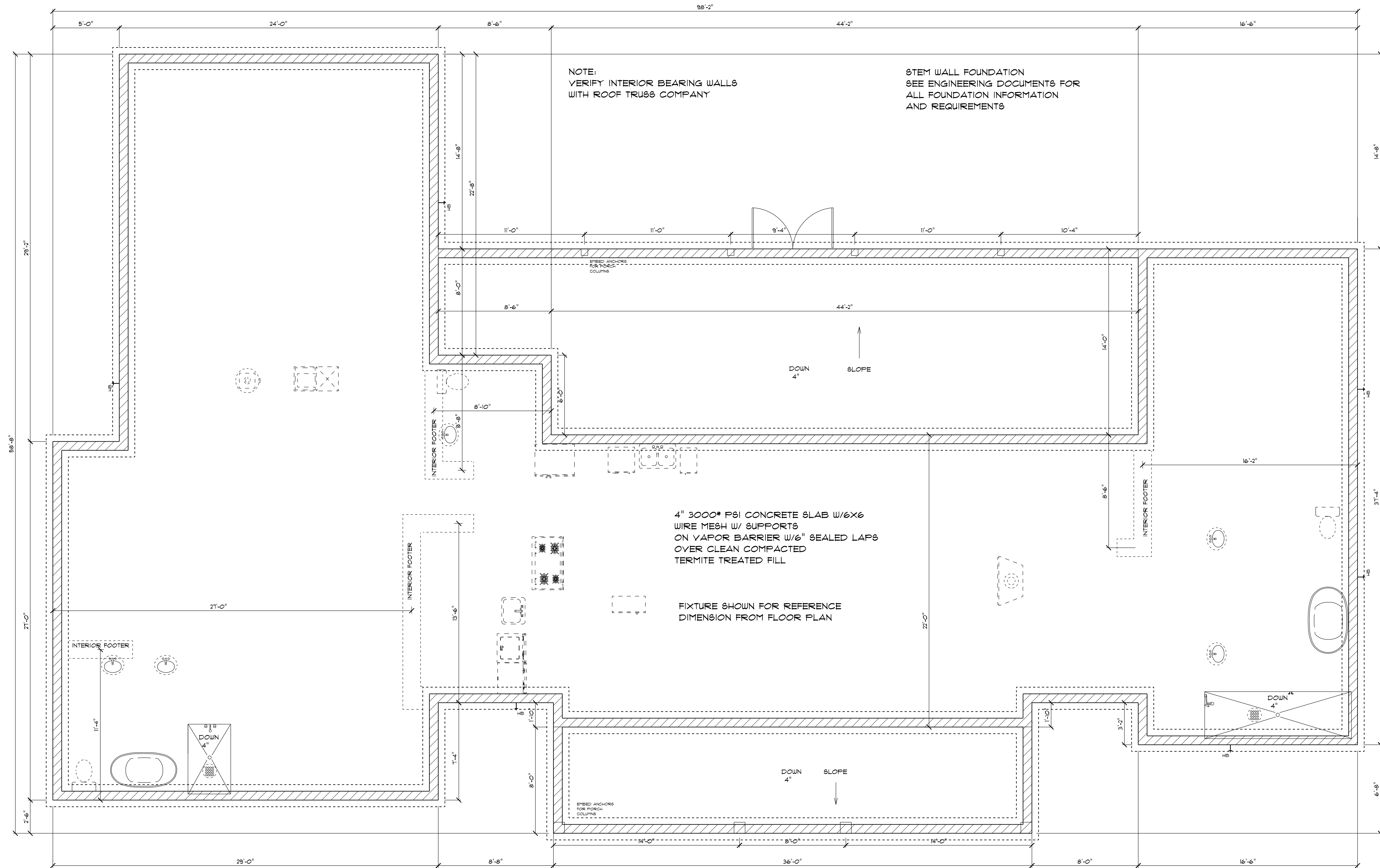
ELECTRICAL PLAN
