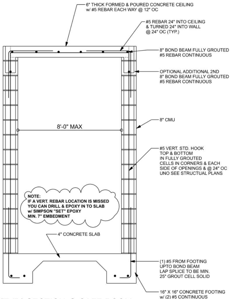
(TYP.) SECTION @ SAFE ROOM ONE STORY CMU
