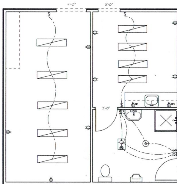
Electrical Plan Mechanical Room Break Room Bath Room
