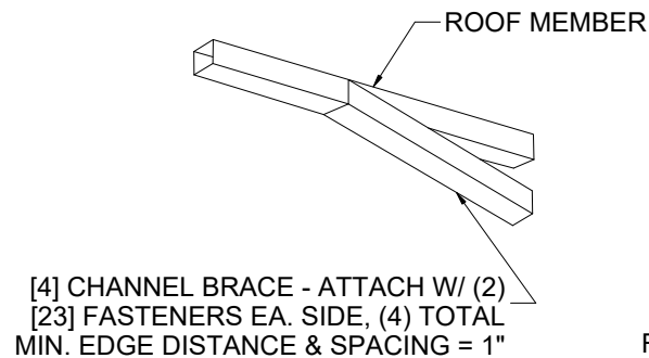
2. PEAK BRACE CONNECTION DETAILS
