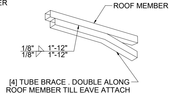
2. PEAK BRACE CONNECTION DETAILS
