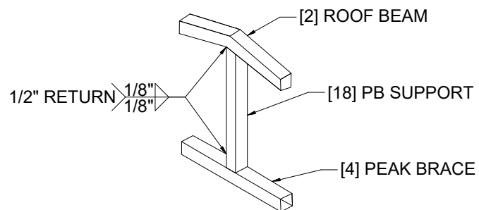
4. PB SUPPORT DETAIL
