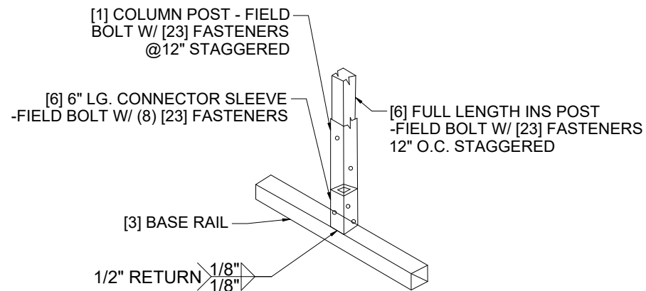
3. BASE DETAIL
